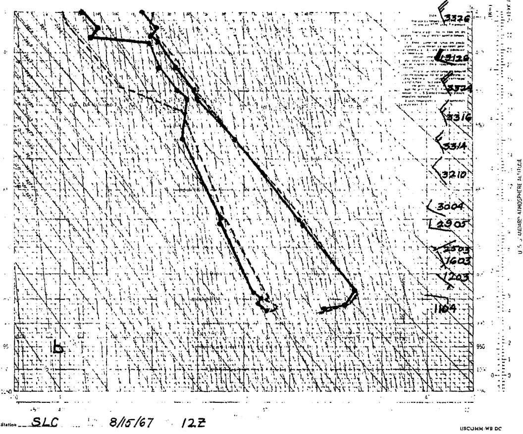
Figure 8: Salt Lake City Raobs 1200Z August 14 and 15, 1967. Dashed line in Figure 8 is sounding for 1200Z August 15.
