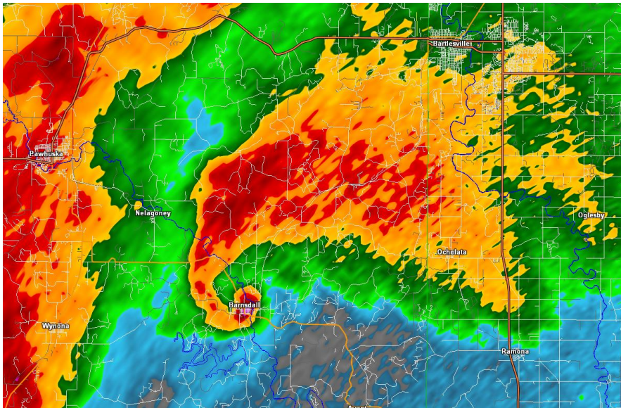
Barnsdall, OK Tornadic Supercell with debris ball, May 6, 2024
