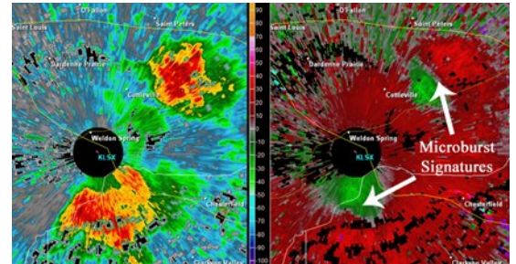
Figure 3. Pulse Thunderstorms
