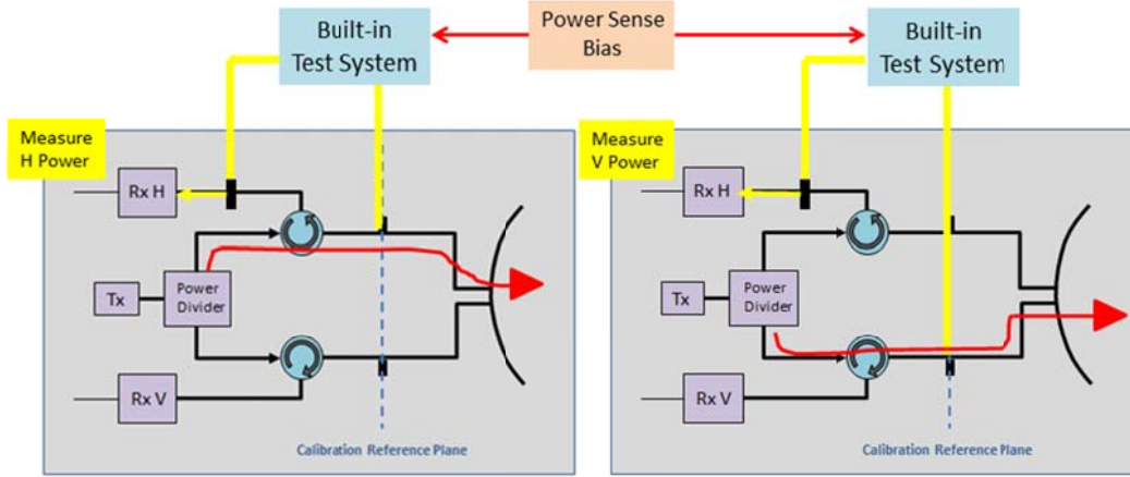
Figure 8: Transmitter Power Bias Measurement
