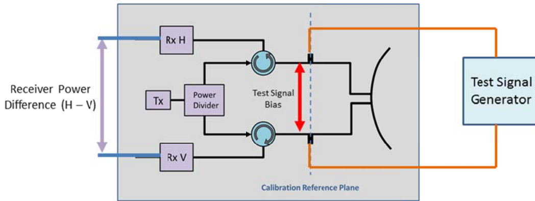
Figure 5: Receiver Bias Measurement
