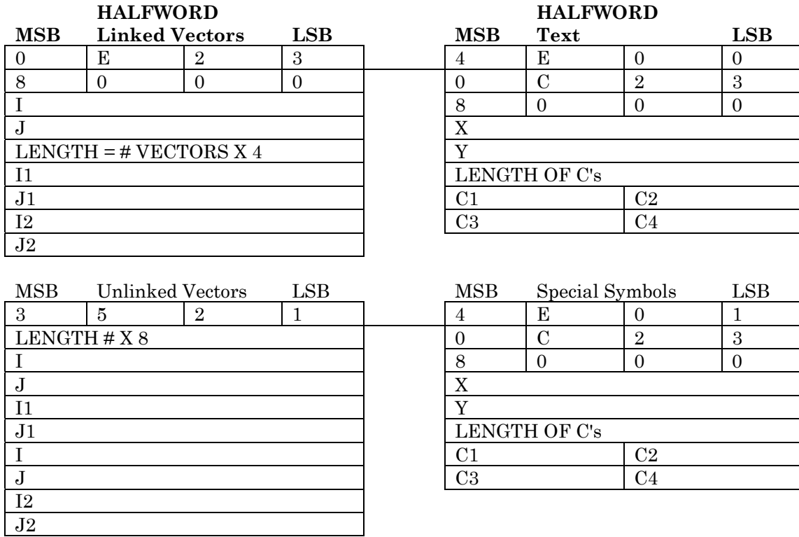
Figure 3-9. Map Message Packet - Packet Codes 0E23, 4E00, 3521 and 4E01 (Sheet 2)
