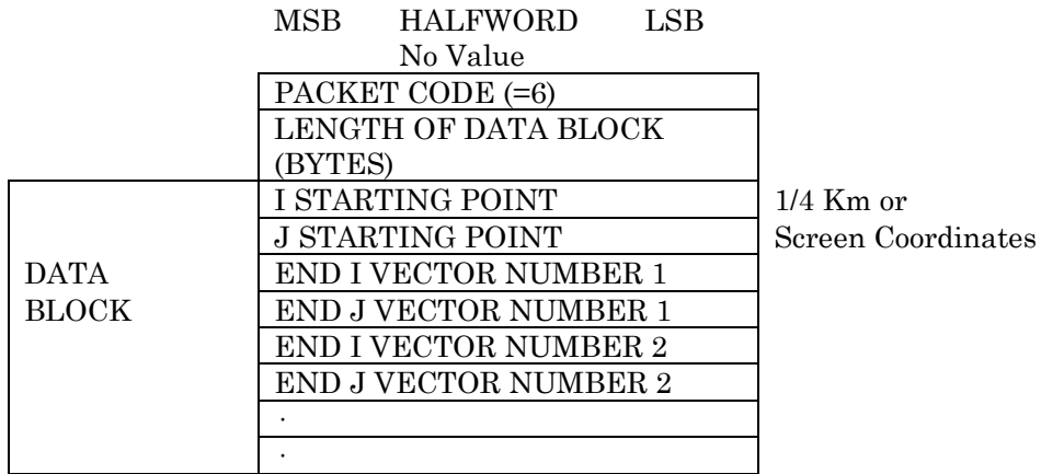
Figure 3-7 Linked Vector Packet - Packet Code 6 (Sheet 1)
