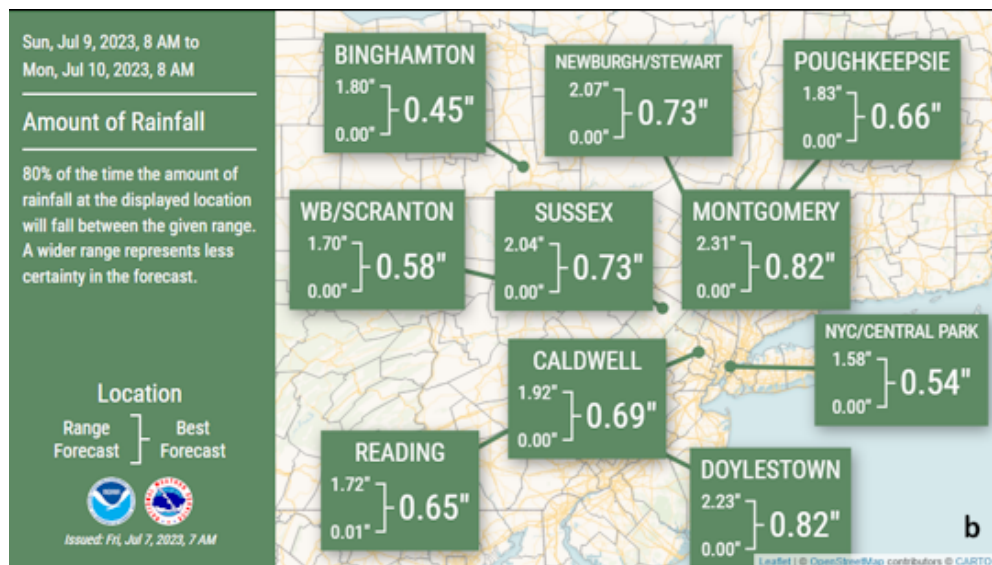
Figure A3. a) QPF probability of exceeding 1.5 inches. b) Probabilistic QPF graphic depicting the high end (90th percentile), most likely, and low end (10th percentile) forecasts.
