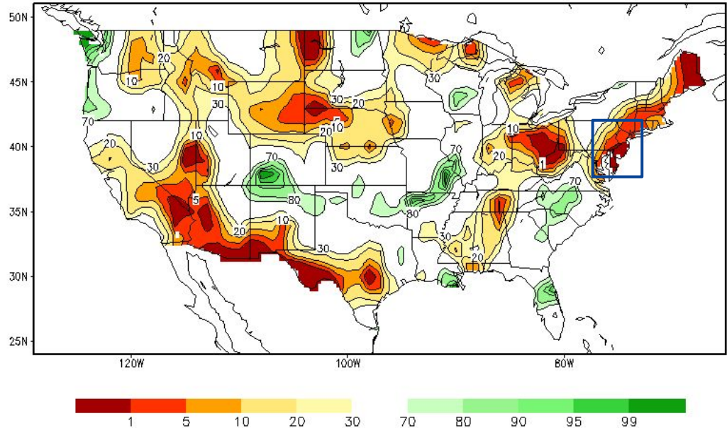
Calculated Soil Moisture Ranking Percentile NOV 07, 2024
