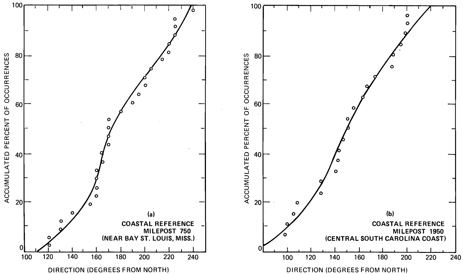
Figure 26.--Landfalling hurricanes and tropical storms, direction of motion vs. cumulative percent of occurrences, (a) Gulf of Mexico (milepost 750) near Bay St. Louis, Miss., (b) east coast (milepost 1950) along central South Carolina coast.
