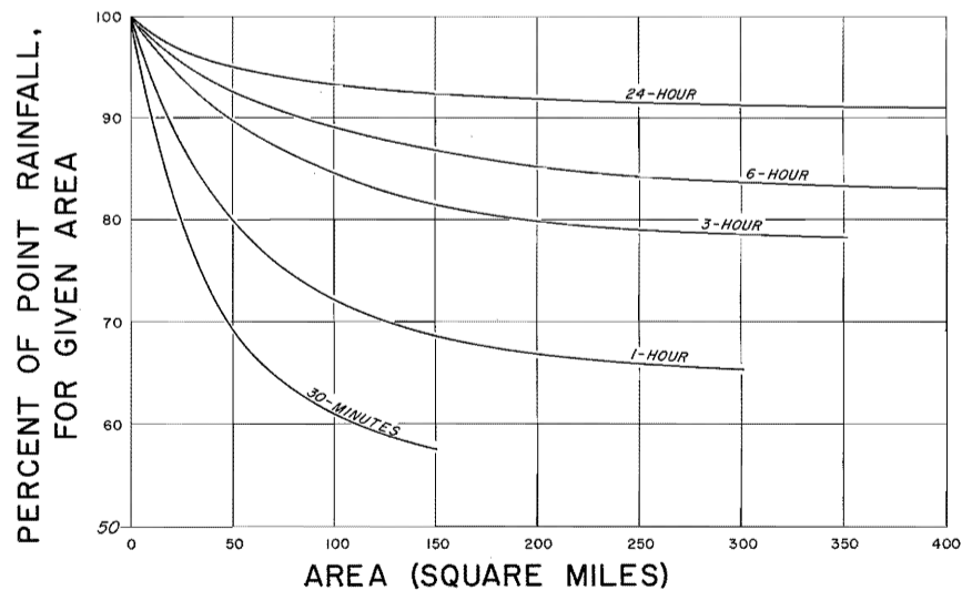
AREA-DEPTH CURVES
