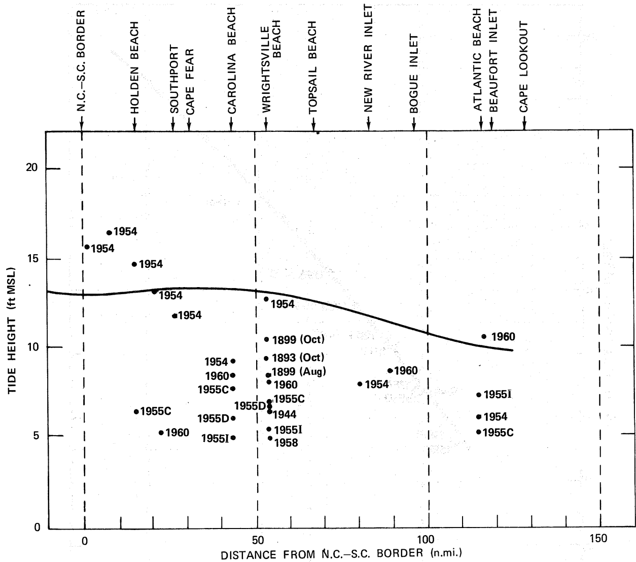
Figure 11.--Representative high-water marks compared with tide frequencies for the 100-yr return period.
