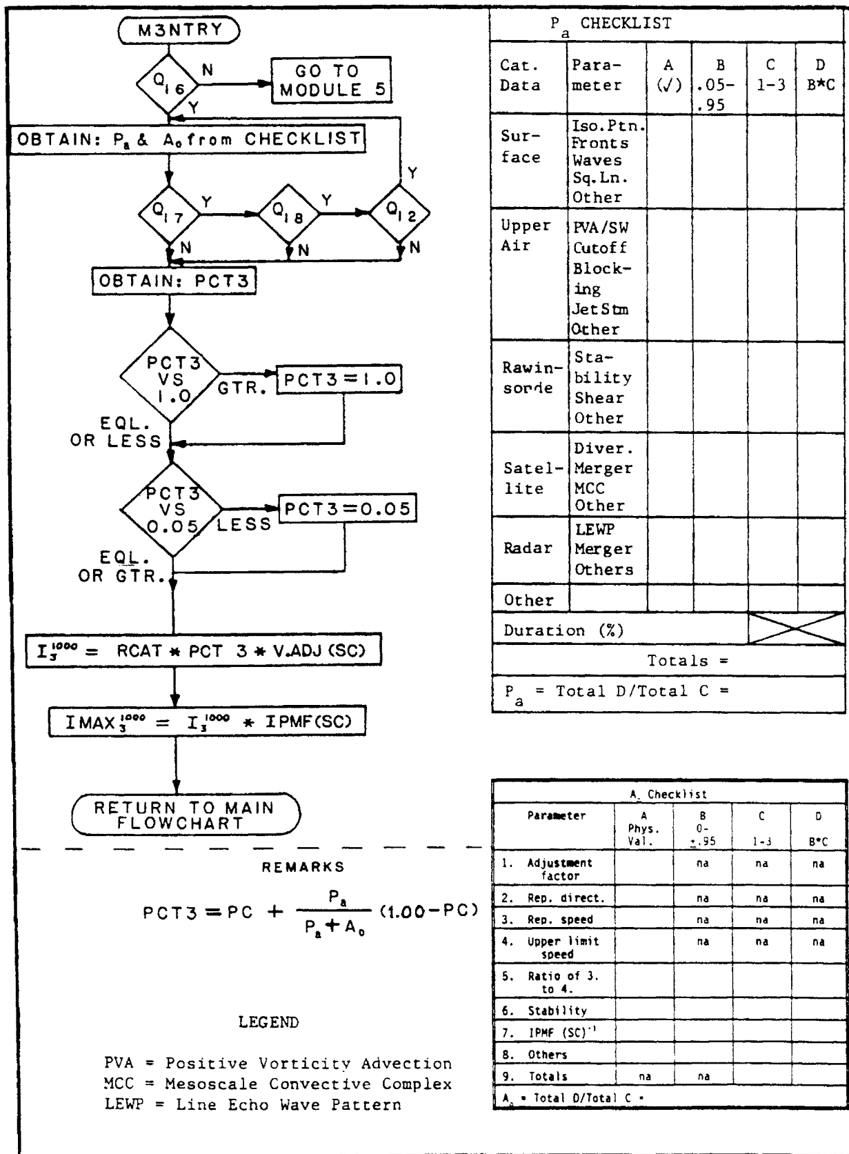
Figure 6.3 -- Module 3 flowchart.
