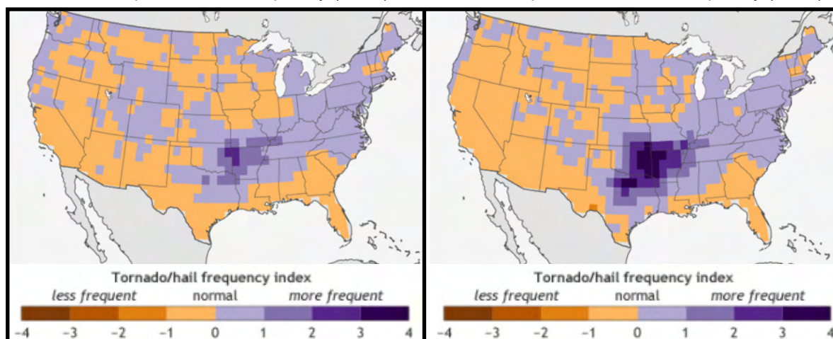
La Niña Impact on Hail Frequency (MAM)
