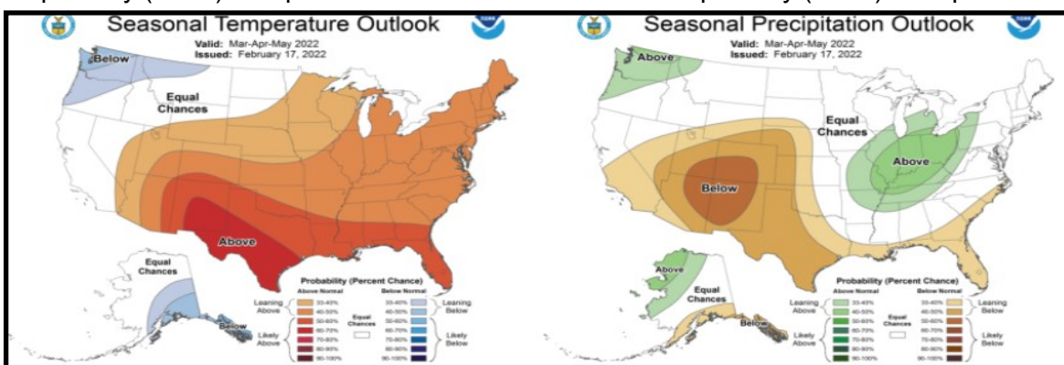
March-April-May (MAM) Temperature Outlook
