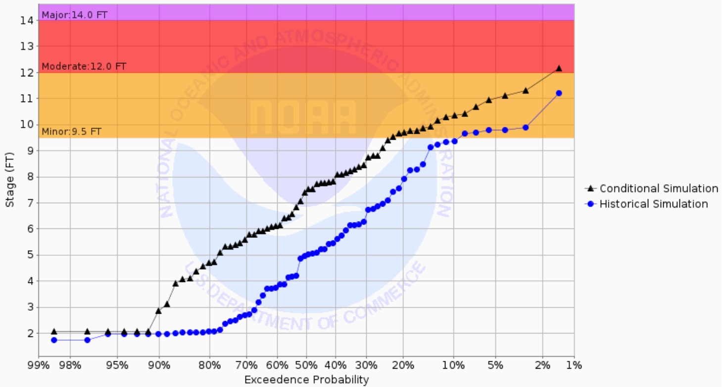
Chance of Exceeding River Stage at Maple River at Enderlin 1E (ENDN8) Forecast for the period 12/30/2024 - 03/30/2025 This is a conditional simulation based on the conditions as of 12/23/2024
