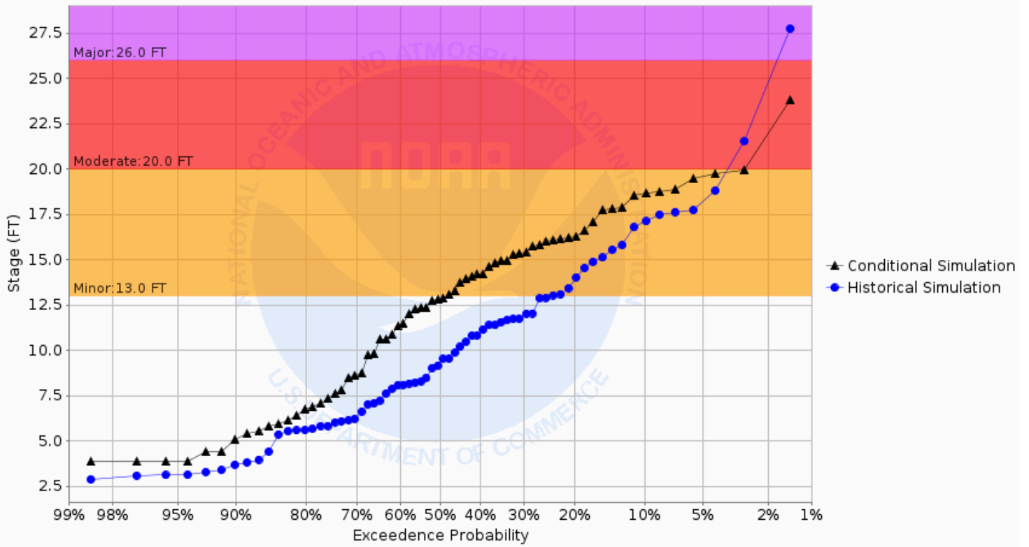
Chance of Exceeding River Stage at Buffalo River at Dilworth 7NE (DILM5) Forecast for the period 12/30/2024 - 03/30/2025 This is a conditional simulation based on the conditions as of 12/23/2024
