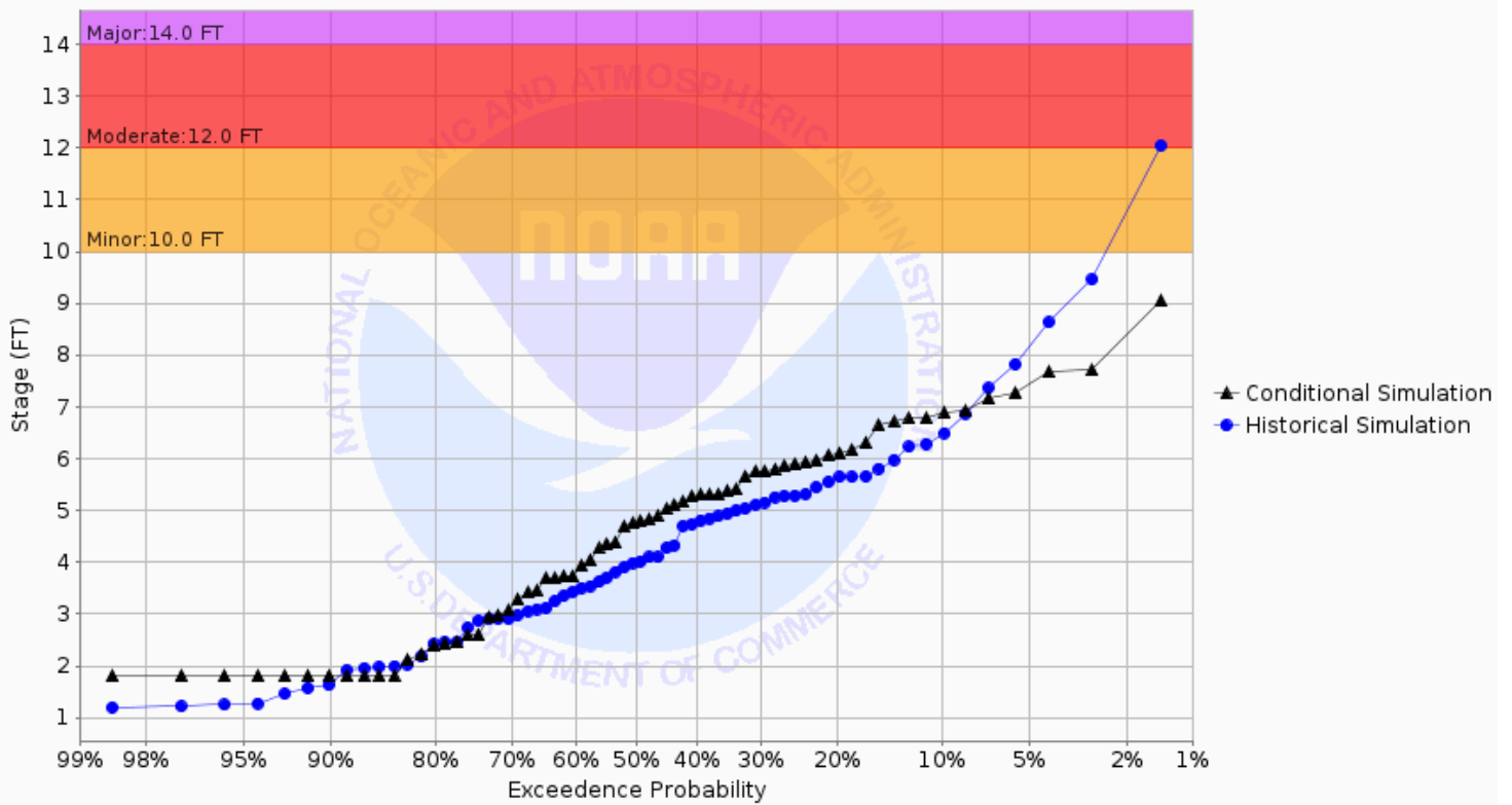
Chance of Exceeding River Stage at Wild Rice River at Twin Valley 1NE (TWVM5) Forecast for the period 12/30/2024 - 03/30/2025 This is a conditional simulation based on the conditions as of 12/23/2024
