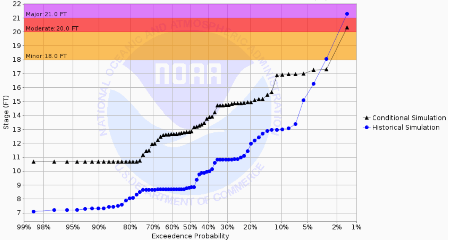
Chance of Exceeding River Stage at Sheyenne River Diversion at West Fargo (WFON8) Forecast for the period 12/30/2024 - 03/30/2025 This is a conditional simulation based on the conditions as of 12/23/2024
