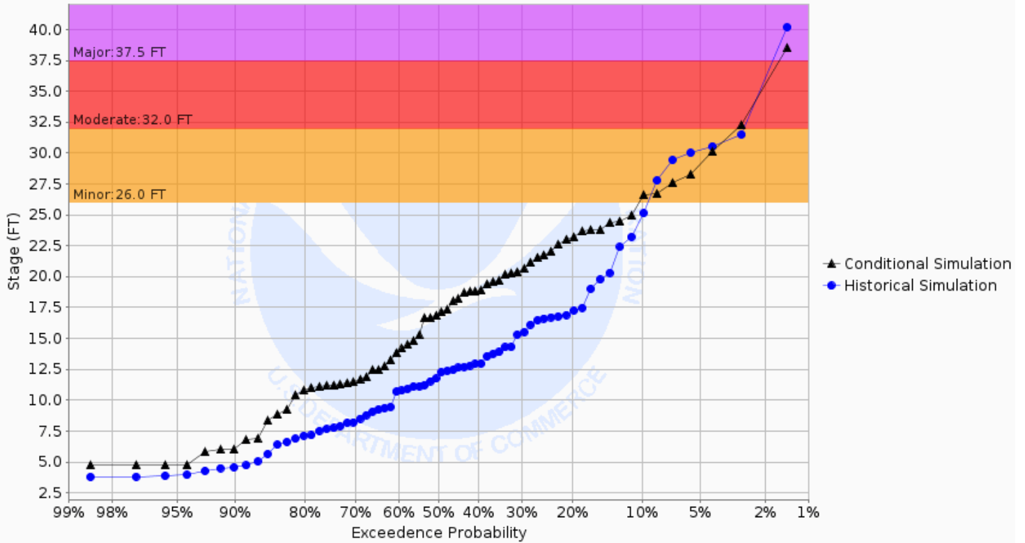
Chance of Exceeding River Stage at Red River of the North at Hillsboro 11ESE (Halstad MN) (HILN8) Forecast for the period 12/30/2024 - 03/30/2025 This is a conditional simulation based on the conditions as of 12/23/2024
