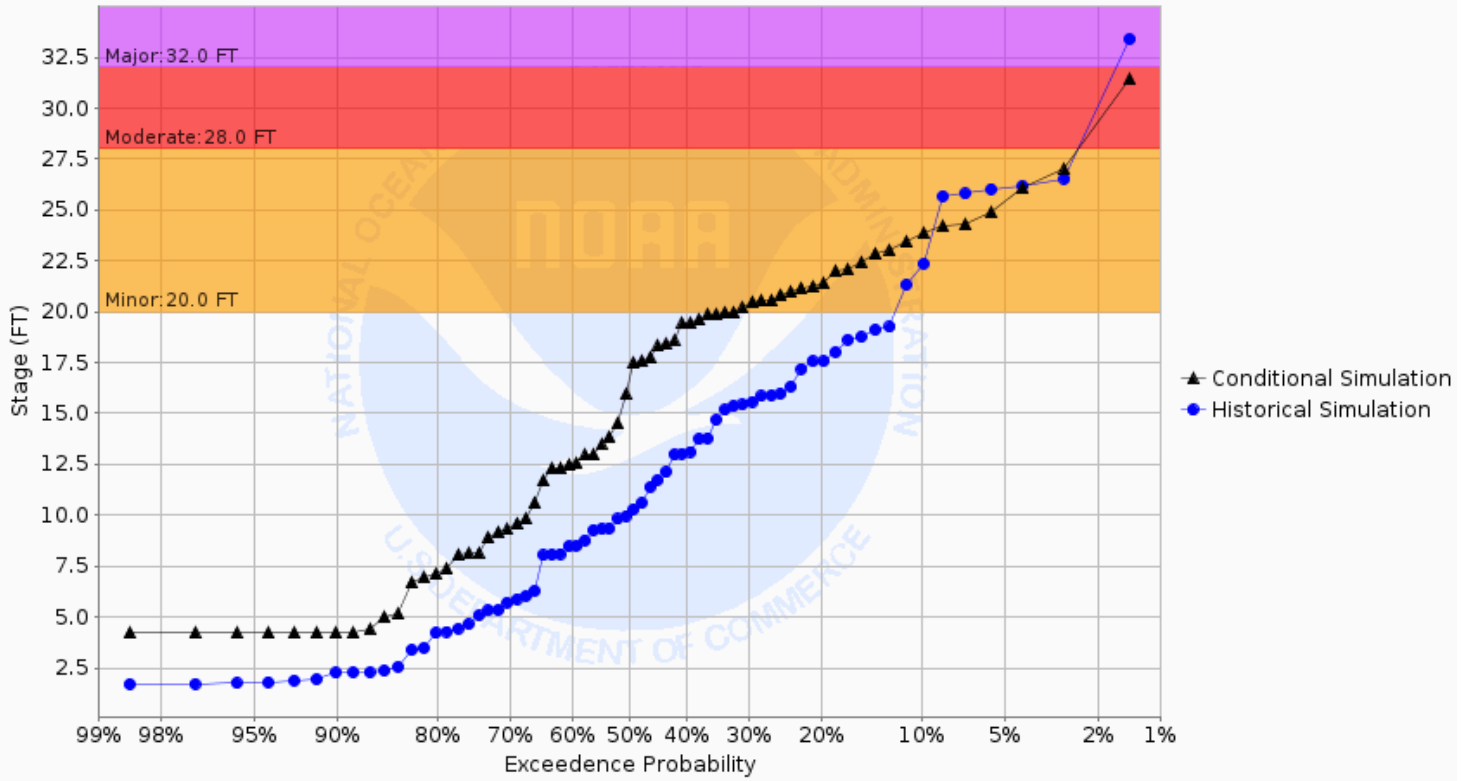
Chance of Exceeding River Stage at Wild Rice River at Hendrum (HNDM5) Forecast for the period 12/30/2024 - 03/30/2025 This is a conditional simulation based on the conditions as of 12/23/2024
