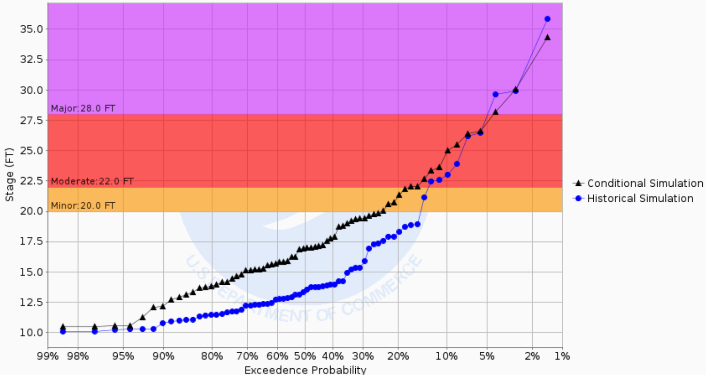
Chance of Exceeding River Stage at Wild Rice River at Abercrombie 2WNW (ABRN8) Forecast for the period 12/30/2024 - 03/30/2025 This is a conditional simulation based on the conditions as of 12/23/2024
