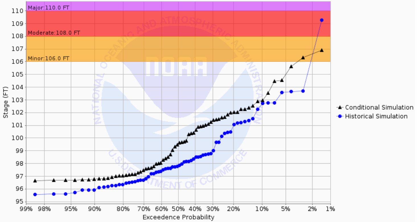
Chance of Exceeding River Stage at Snake River at Alvarado (ALVM5) Forecast for the period 12/30/2024 - 03/30/2025 This is a conditional simulation based on the conditions as of 12/23/2024
