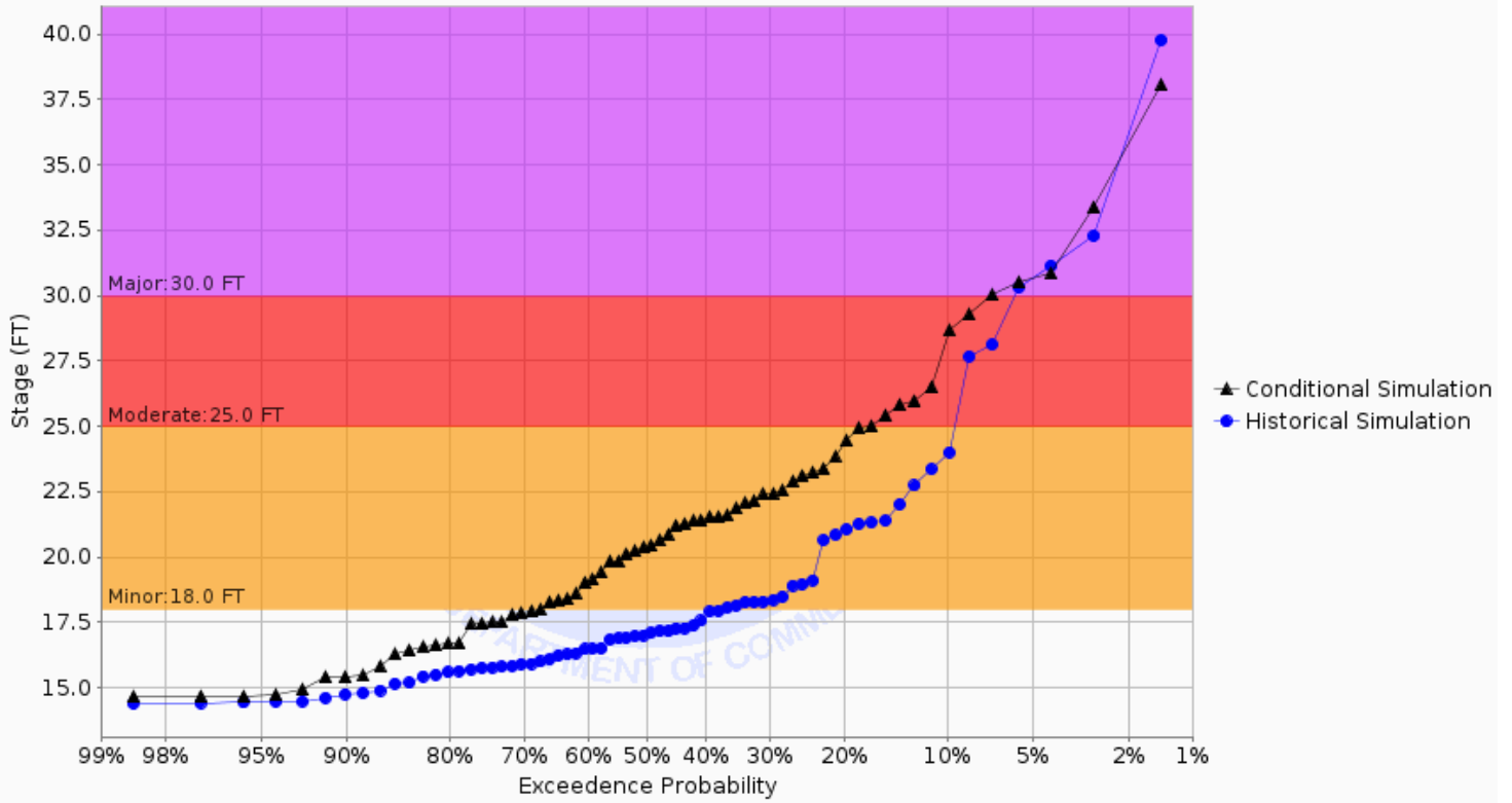
Chance of Exceeding River Stage at Red River of the North at Fargo WTP (FGON8) Forecast for the period 12/30/2024 - 03/30/2025 This is a conditional simulation based on the conditions as of 12/23/2024
