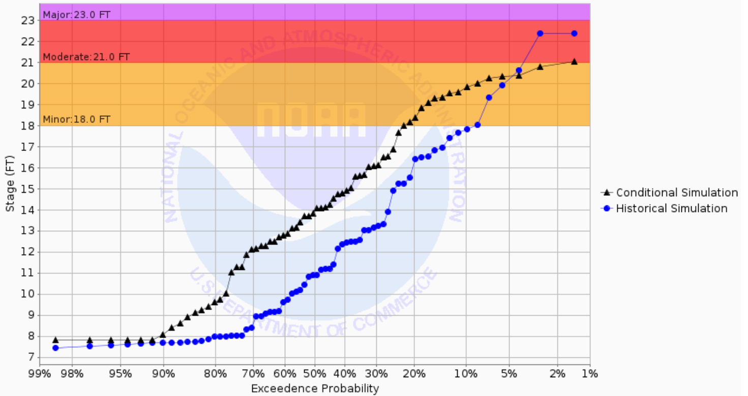
Chance of Exceeding River Stage at Maple River at Mapleton 3SW (MPLN8) Forecast for the period 12/30/2024 - 03/30/2025 This is a conditional simulation based on the conditions as of 12/23/2024
