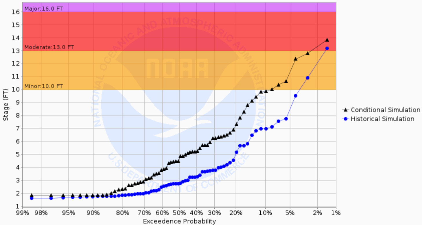
Chance of Exceeding River Stage at Goose River at Hillsboro (HGRN8) Forecast for the period 12/30/2024 - 03/30/2025 This is a conditional simulation based on the conditions as of 12/23/2024
