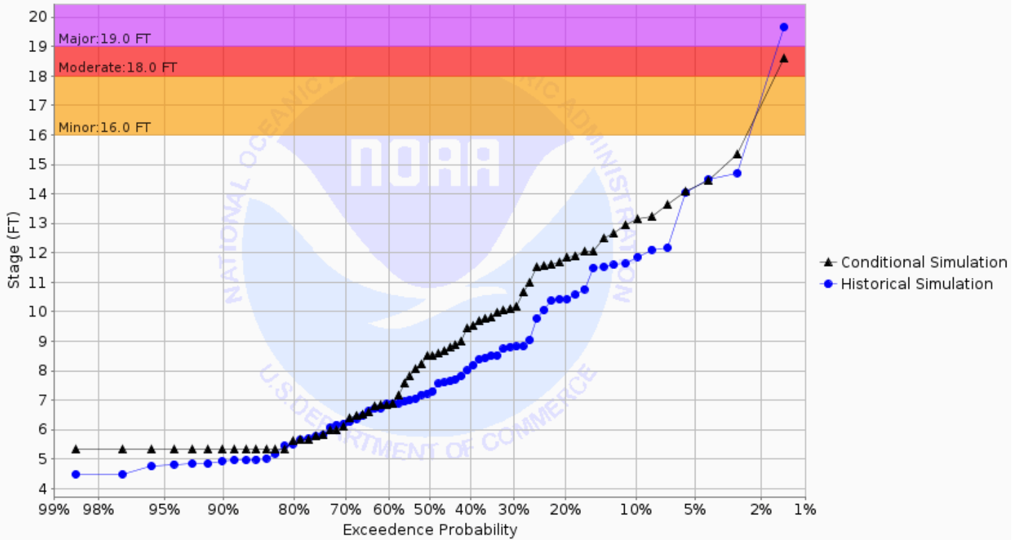
Chance of Exceeding River Stage at Roseau River at Roseau - Center St Brdg (ROSM5) Forecast for the period 12/30/2024 - 03/30/2025 This is a conditional simulation based on the conditions as of 12/23/2024
