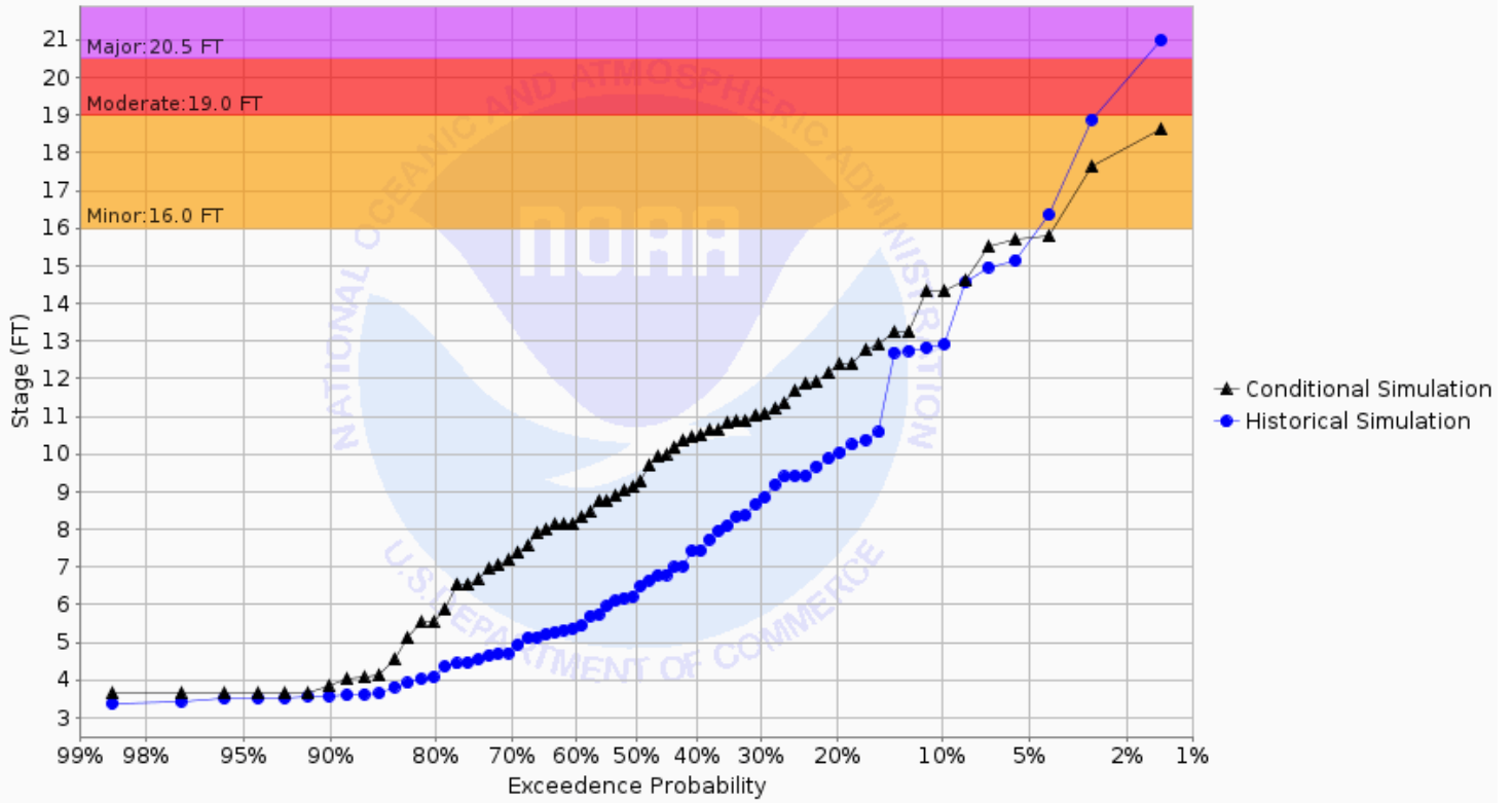
Chance of Exceeding River Stage at Sheyenne River at Kindred 2SE (KNDN8) Forecast for the period 12/30/2024 - 03/30/2025 This is a conditional simulation based on the conditions as of 12/23/2024
