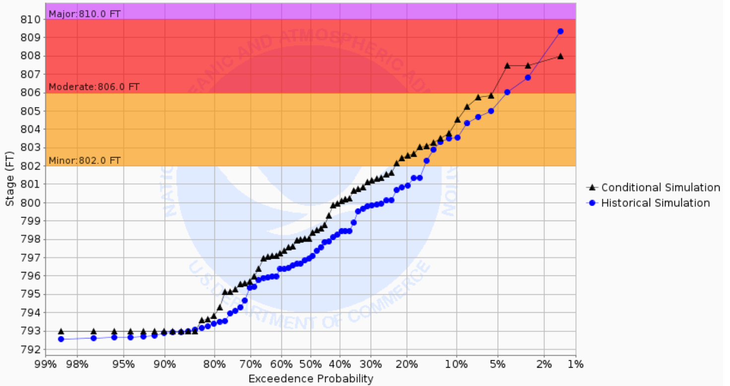
Chance of Exceeding River Stage at Two Rivers River at Hallock (HLLM5) Forecast for the period 12/30/2024 - 03/30/2025 This is a conditional simulation based on the conditions as of 12/23/2024
