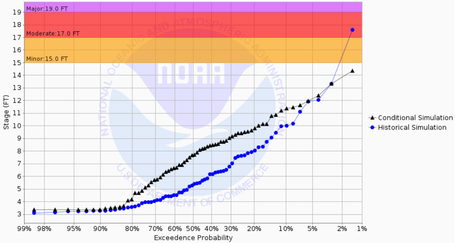
Chance of Exceeding River Stage at Sheyenne River at Lisbon (LBNN8) Forecast for the period 12/30/2024 - 03/30/2025 This is a conditional simulation based on the conditions as of 12/23/2024
