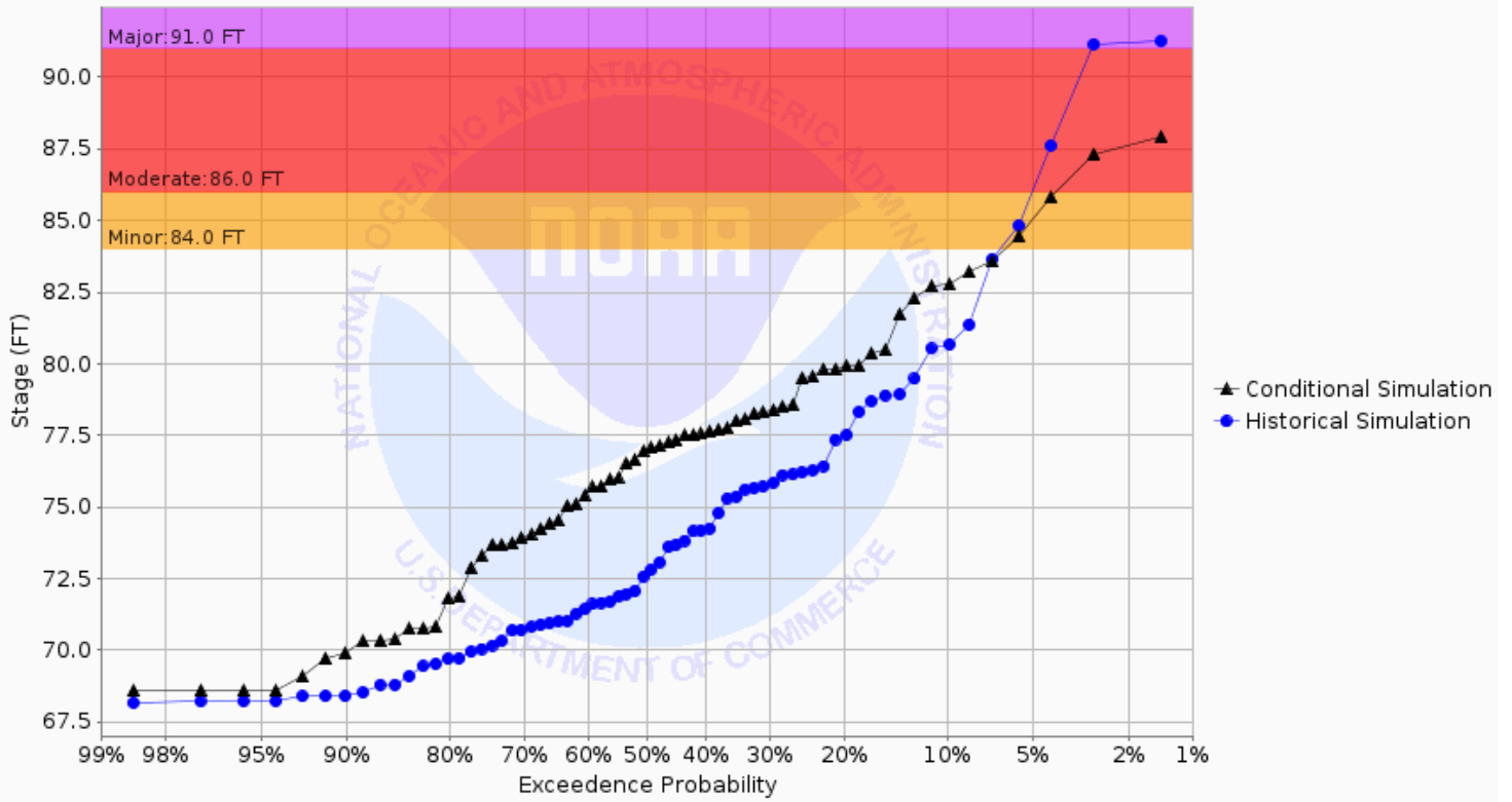
Chance of Exceeding River Stage at Sheyenne River at Harwood (HWDN8) Forecast for the period 12/30/2024 - 03/30/2025 This is a conditional simulation based on the conditions as of 12/23/2024
