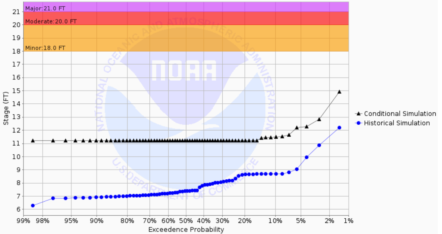
Chance of Exceeding River Stage at Sheyenne River Diversion at West Fargo (WFON8) Forecast for the period 12/02/2024 - 03/02/2025 This is a conditional simulation based on the conditions as of 11/25/2024
