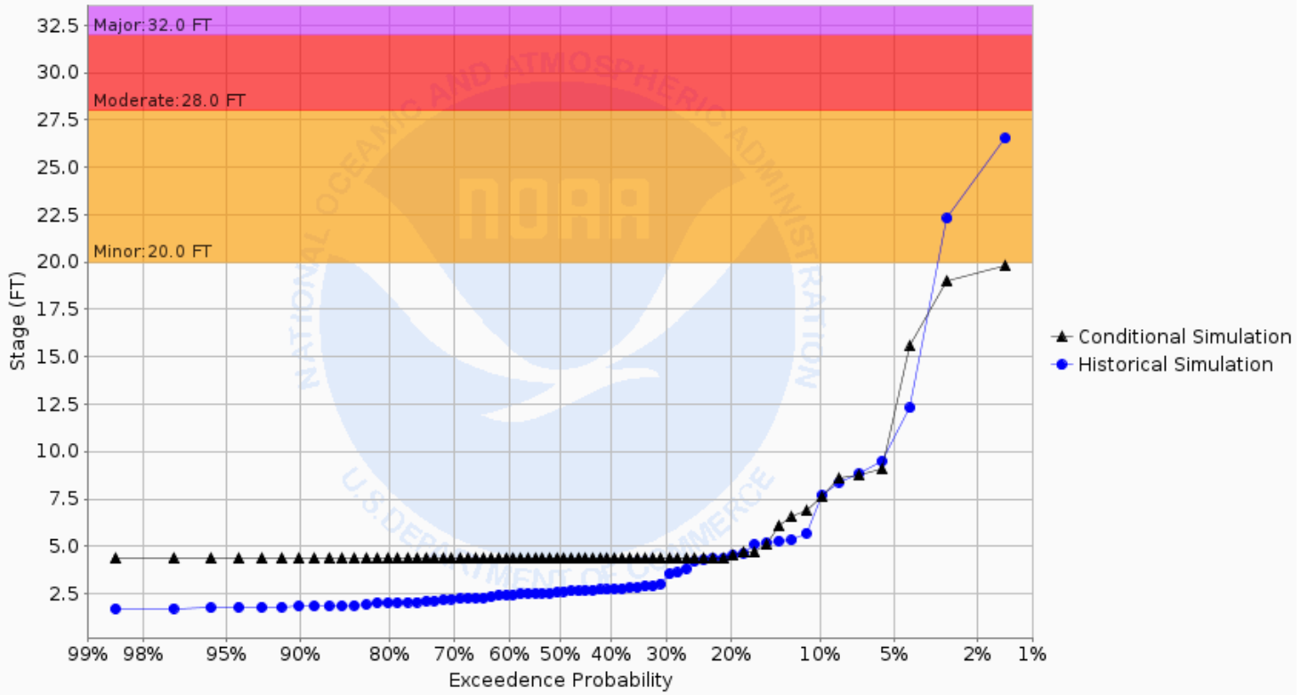
Chance of Exceeding River Stage at Wild Rice River at Hendrum (HNDM5) Forecast for the period 12/02/2024 - 03/02/2025 This is a conditional simulation based on the conditions as of 11/25/2024
