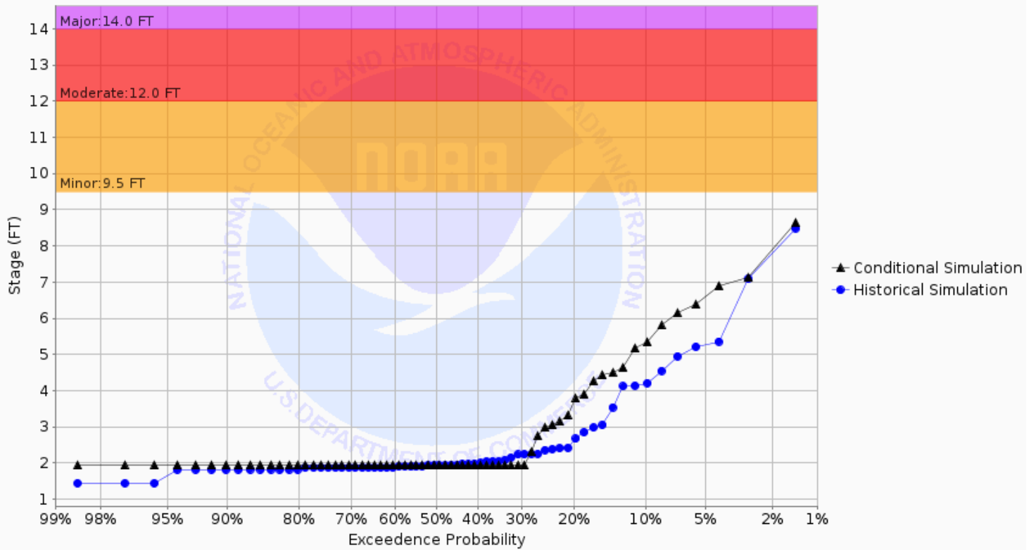
Chance of Exceeding River Stage at Maple River at Enderlin 1E (ENDN8) Forecast for the period 12/02/2024 - 03/02/2025 This is a conditional simulation based on the conditions as of 11/25/2024
