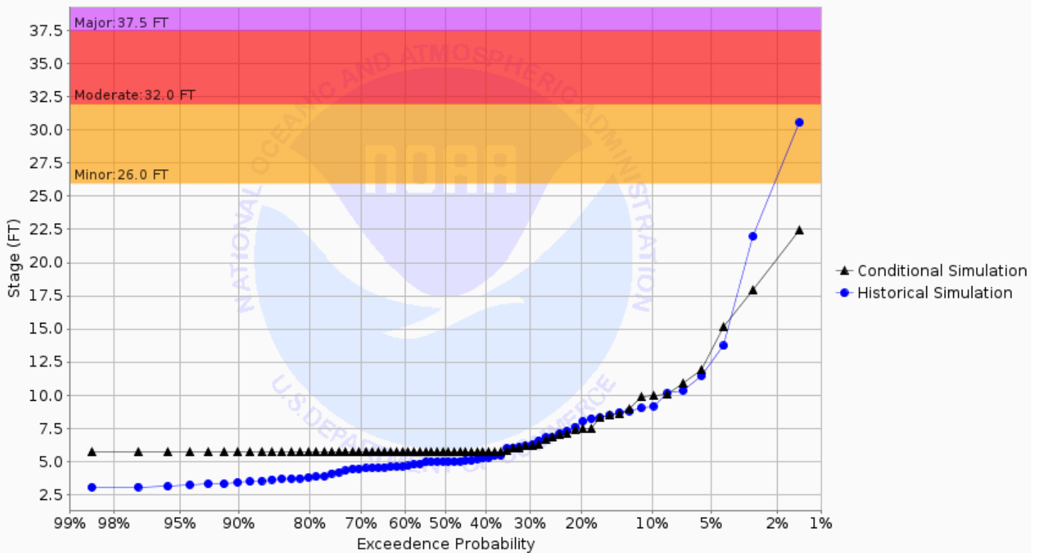
Chance of Exceeding River Stage at Red River of the North at Hillsboro 11ESE (Halstad MN) (HILN8) Forecast for the period 12/02/2024 - 03/02/2025 This is a conditional simulation based on the conditions as of 11/25/2024
