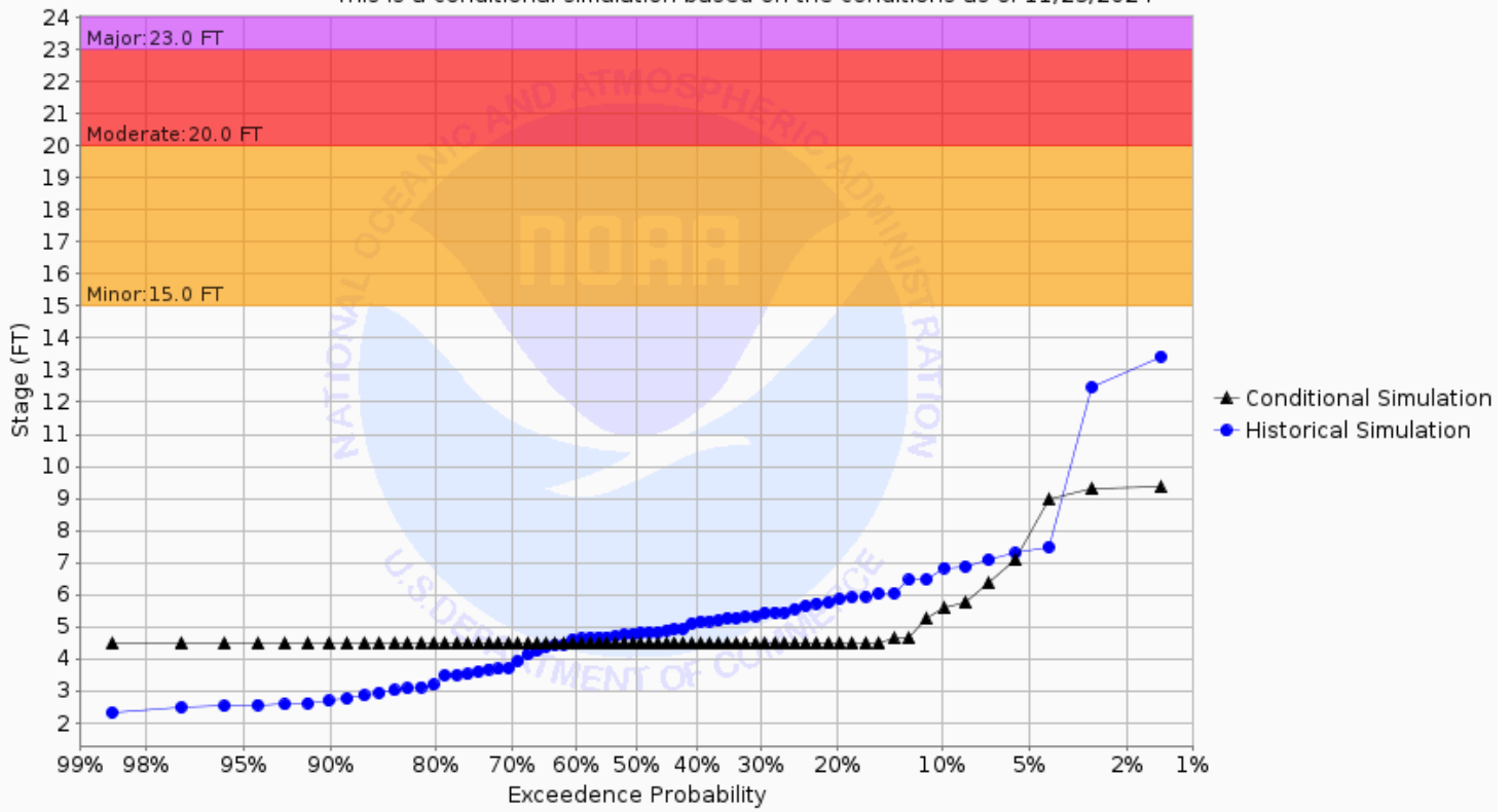
Chance of Exceeding River Stage at Red Lake River at Crookston (CRKM5) Forecast for the period 12/02/2024 - 03/02/2025 This is a conditional simulation based on the conditions as of 11/25/2024
