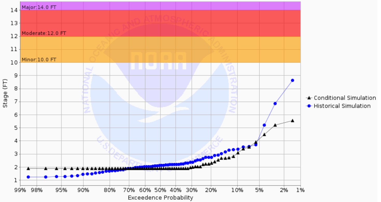
Chance of Exceeding River Stage at Wild Rice River at Twin Valley 1NE (TWVM5) Forecast for the period 12/02/2024 - 03/02/2025 This is a conditional simulation based on the conditions as of 11/25/2024
