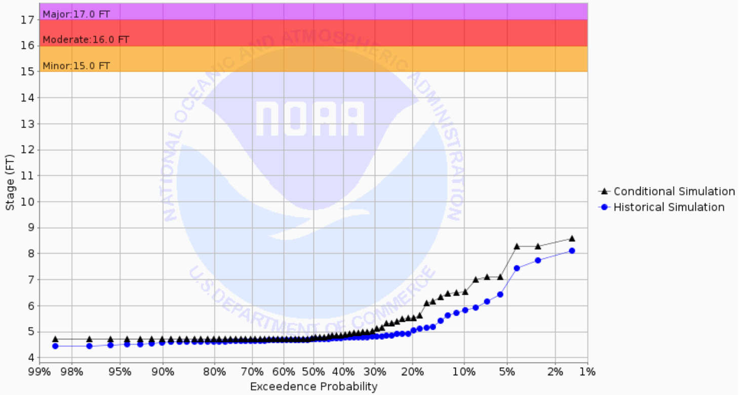
Chance of Exceeding River Stage at Sheyenne River at Valley City (VCRN8) Forecast for the period 12/02/2024 - 03/02/2025 This is a conditional simulation based on the conditions as of 11/25/2024
