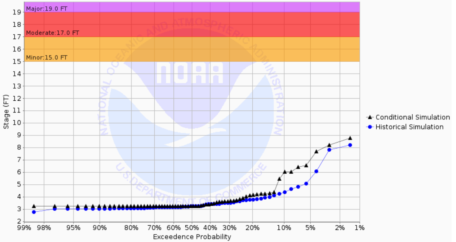
Chance of Exceeding River Stage at Sheyenne River at Lisbon (LBNN8) Forecast for the period 12/02/2024 - 03/02/2025 This is a conditional simulation based on the conditions as of 11/25/2024
