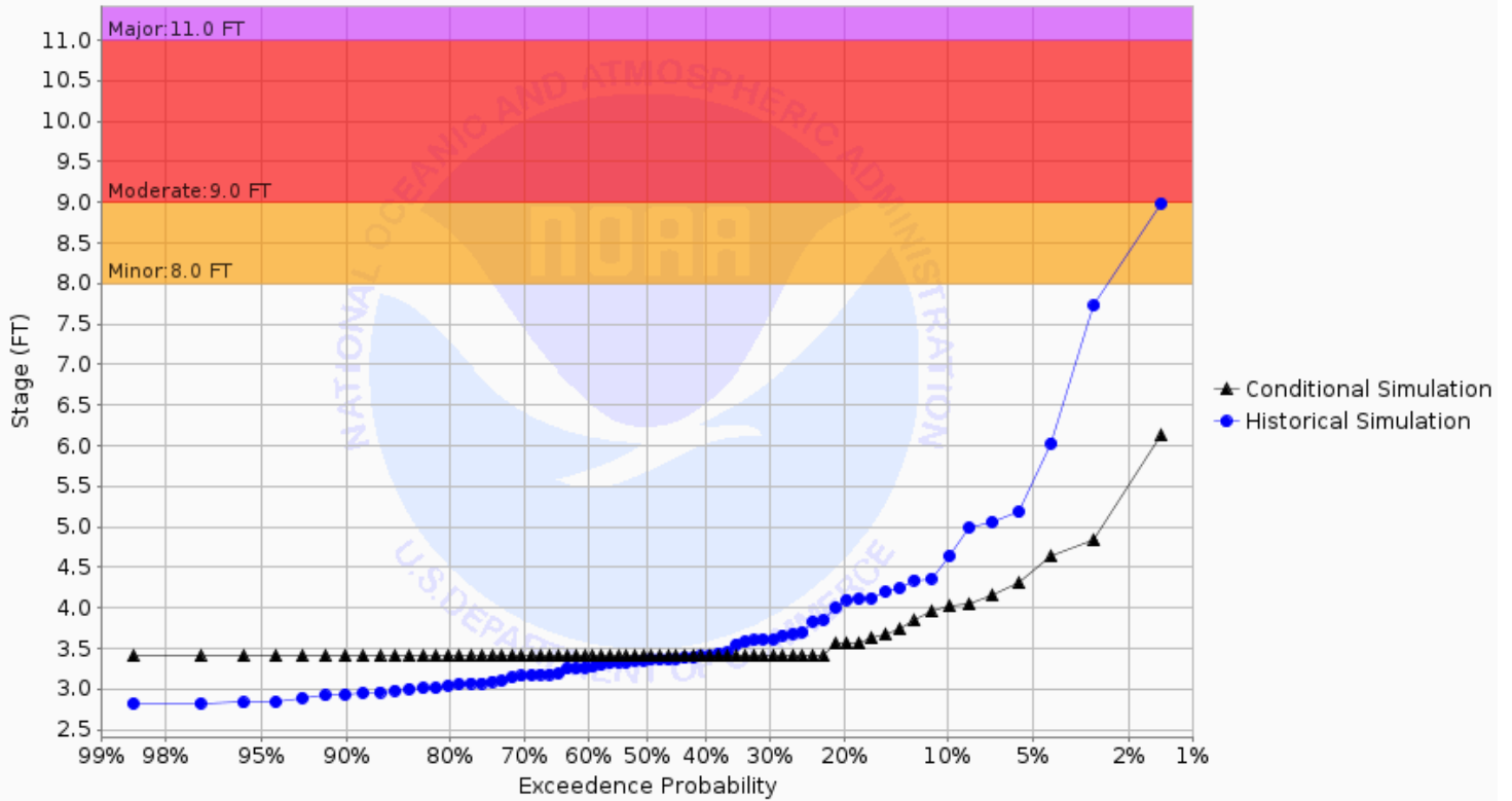
Chance of Exceeding River Stage at Buffalo River at Hawley 2SW (HWYM5) Forecast for the period 12/02/2024 - 03/02/2025 This is a conditional simulation based on the conditions as of 11/25/2024
