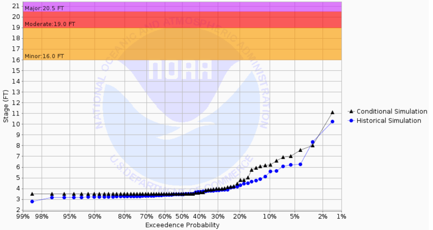
Chance of Exceeding River Stage at Sheyenne River at Kindred 2SE (KNDN8) Forecast for the period 12/02/2024 - 03/02/2025 This is a conditional simulation based on the conditions as of 11/25/2024
