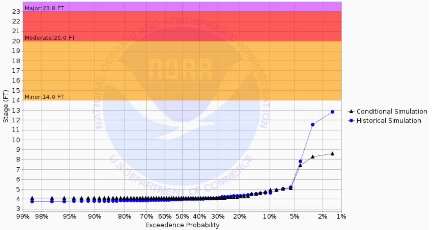
Chance of Exceeding River Stage at Marsh River at Shelly 4SE (SHYM5) Forecast for the period 12/02/2024 - 03/02/2025 This is a conditional simulation based on the conditions as of 11/25/2024
