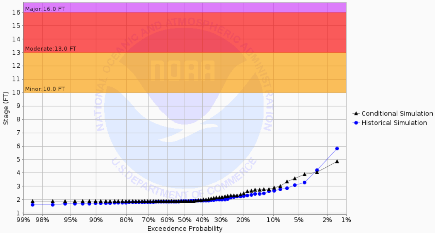
Chance of Exceeding River Stage at Goose River at Hillsboro (HGRN8) Forecast for the period 12/02/2024 - 03/02/2025 This is a conditional simulation based on the conditions as of 11/25/2024
