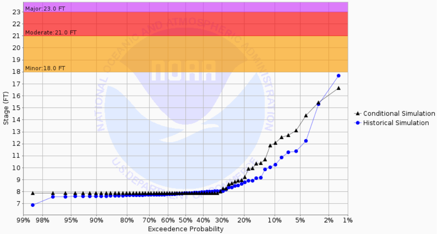
Chance of Exceeding River Stage at Maple River at Mapleton 3SW (MPLN8) Forecast for the period 12/02/2024 - 03/02/2025 This is a conditional simulation based on the conditions as of 11/25/2024
