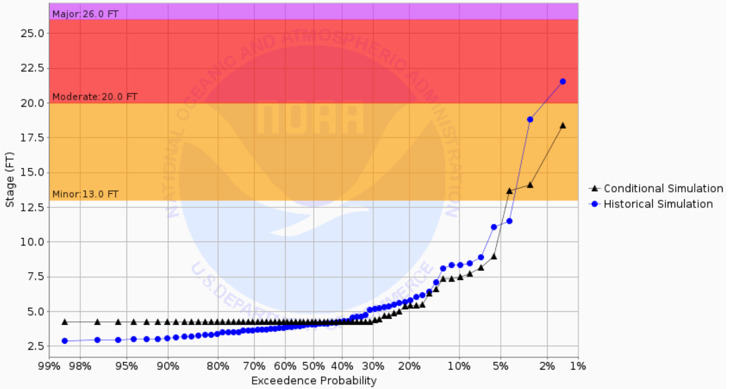
Chance of Exceeding River Stage at Buffalo River at Dilworth 7NE (DILM5) Forecast for the period 12/02/2024 - 03/02/2025 This is a conditional simulation based on the conditions as of 11/25/2024
