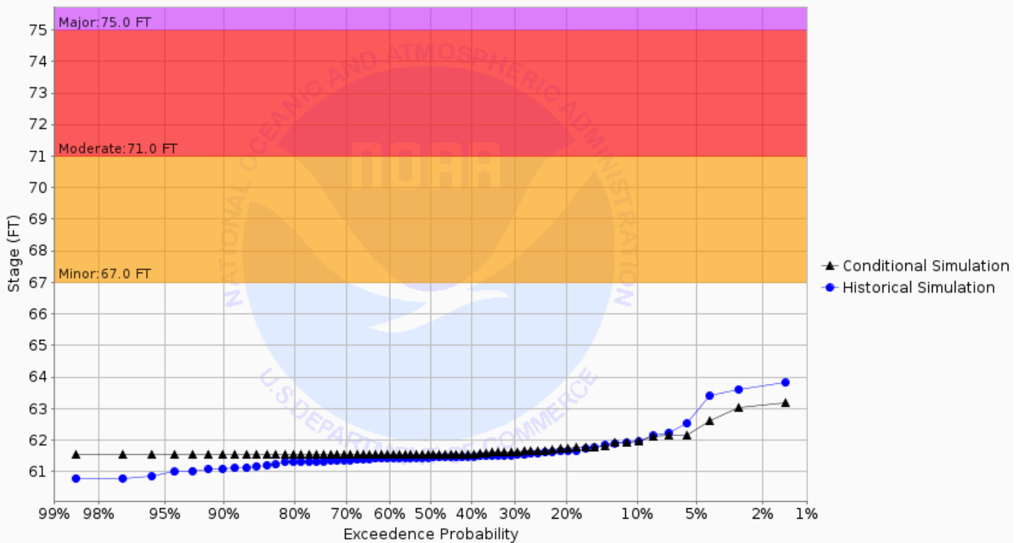
Chance of Exceeding River Stage at Snake River at Warren 3ENE-Morkassel Brdg (MKLM5) Forecast for the period 12/02/2024 - 03/02/2025 This is a conditional simulation based on the conditions as of 11/25/2024
