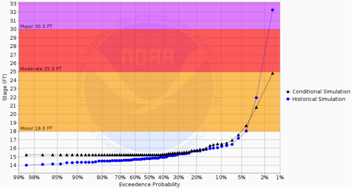
Chance of Exceeding River Stage at Red River of the North at Fargo WTP (FGON8) Forecast for the period 12/02/2024 - 03/02/2025 This is a conditional simulation based on the conditions as of 11/25/2024
