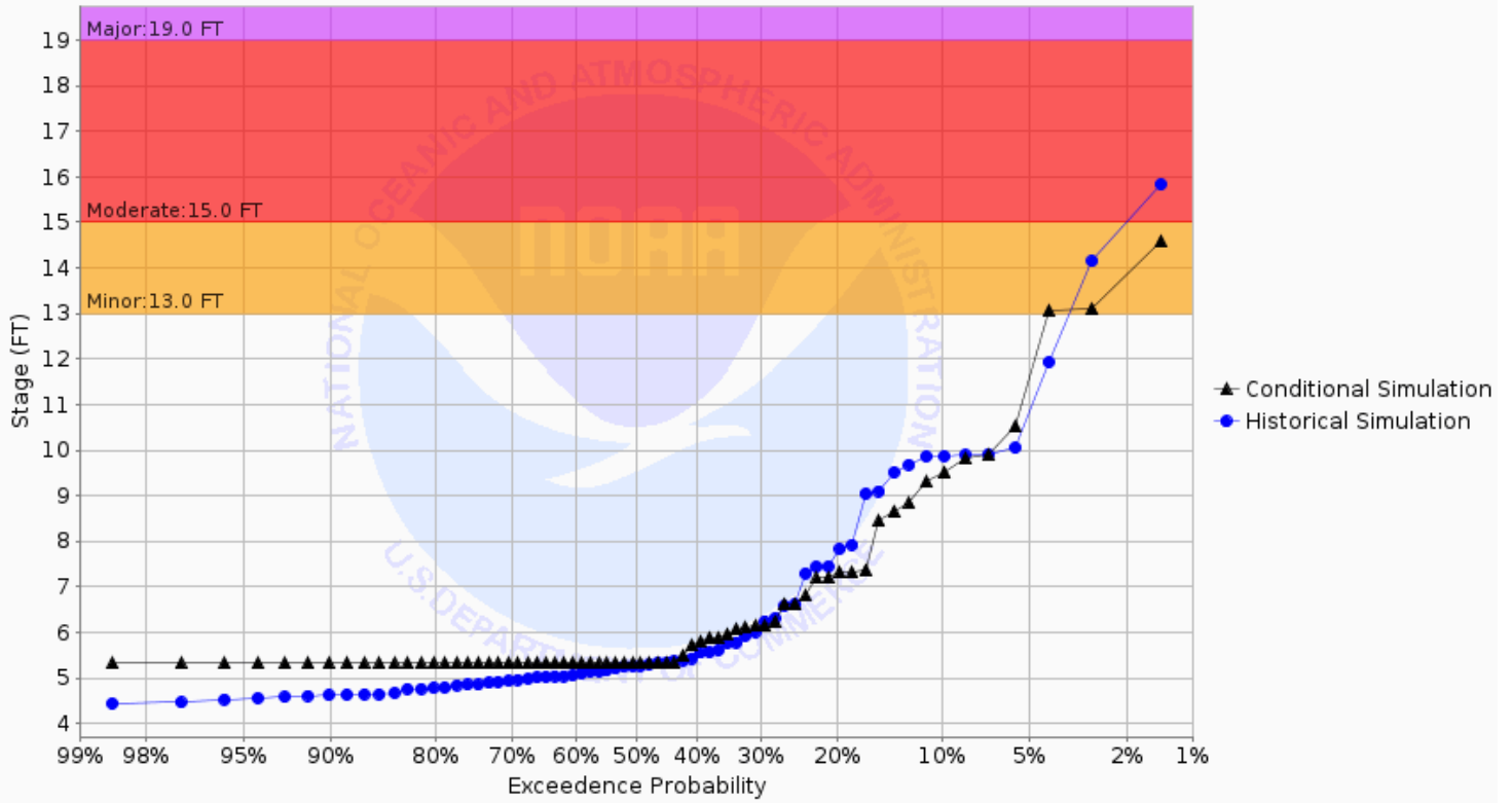
Chance of Exceeding River Stage at South Branch Buffalo River at Sabin 1E (SABM5) Forecast for the period 12/02/2024 - 03/02/2025 This is a conditional simulation based on the conditions as of 11/25/2024
