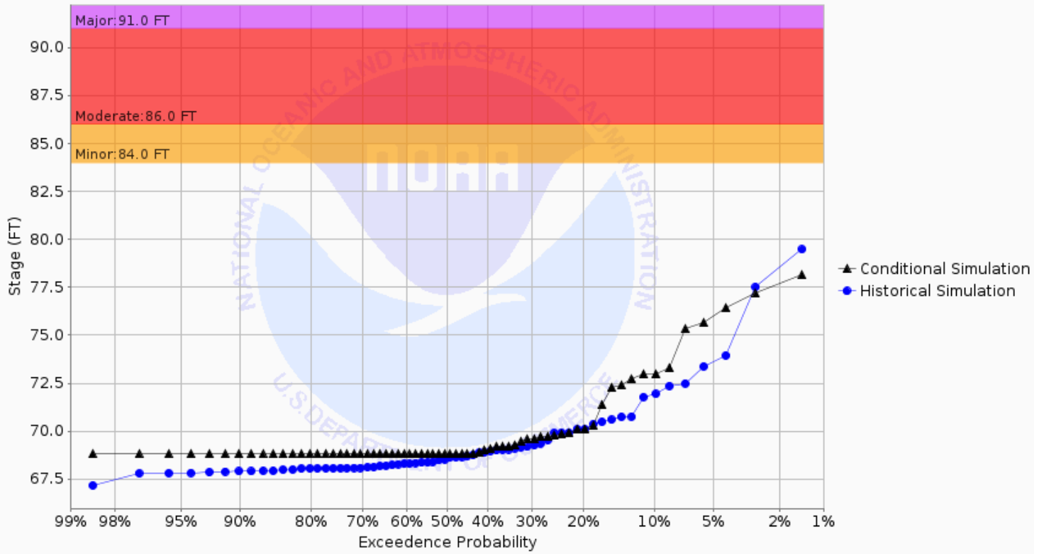
Chance of Exceeding River Stage at Sheyenne River at Harwood (HWDN8) Forecast for the period 12/02/2024 - 03/02/2025 This is a conditional simulation based on the conditions as of 11/25/2024
