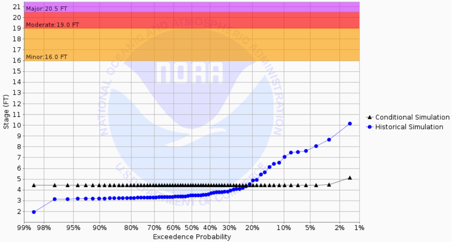
Chance of Exceeding River Stage at Sheyenne River at Kindred 2SE (KNDN8) Forecast for the period 10/28/2024 - 01/26/2025 This is a conditional simulation based on the conditions as of 10/21/2024
