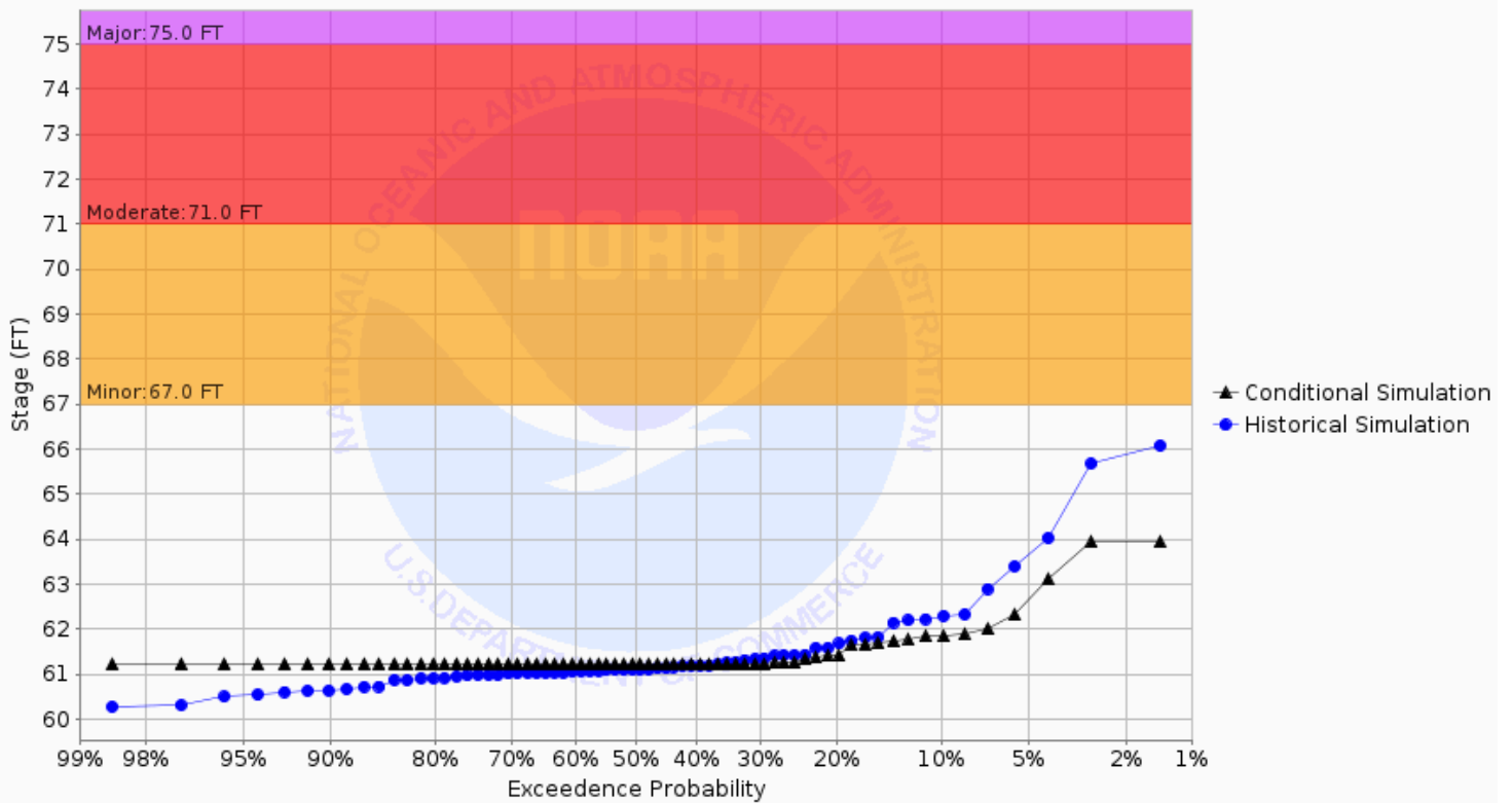
Chance of Exceeding River Stage at Snake River at Warren 3ENE-Morkassel Brdg (MKLM5) Forecast for the period 10/28/2024 - 01/26/2025 This is a conditional simulation based on the conditions as of 10/21/2024
