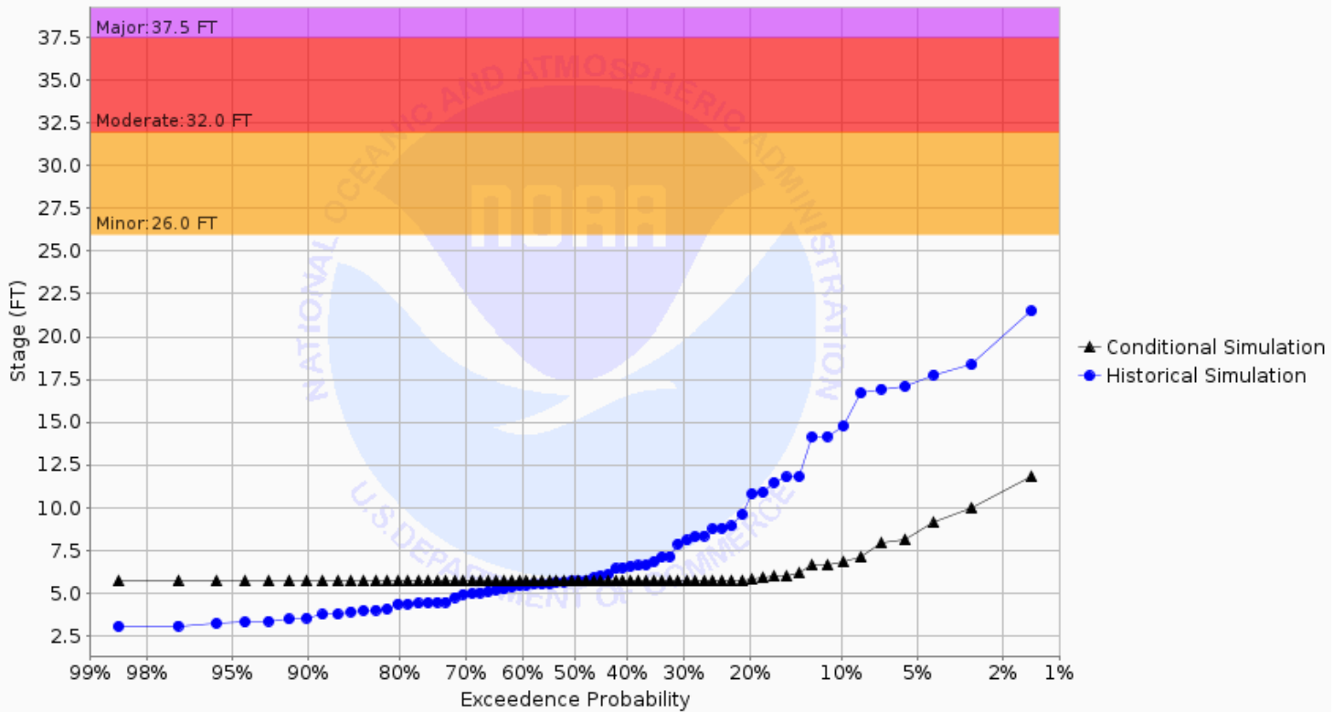
Chance of Exceeding River Stage at Red River of the North at Hillsboro 11ESE (Halstad MN) (HILN8) Forecast for the period 10/28/2024 - 01/26/2025 This is a conditional simulation based on the conditions as of 10/21/2024
