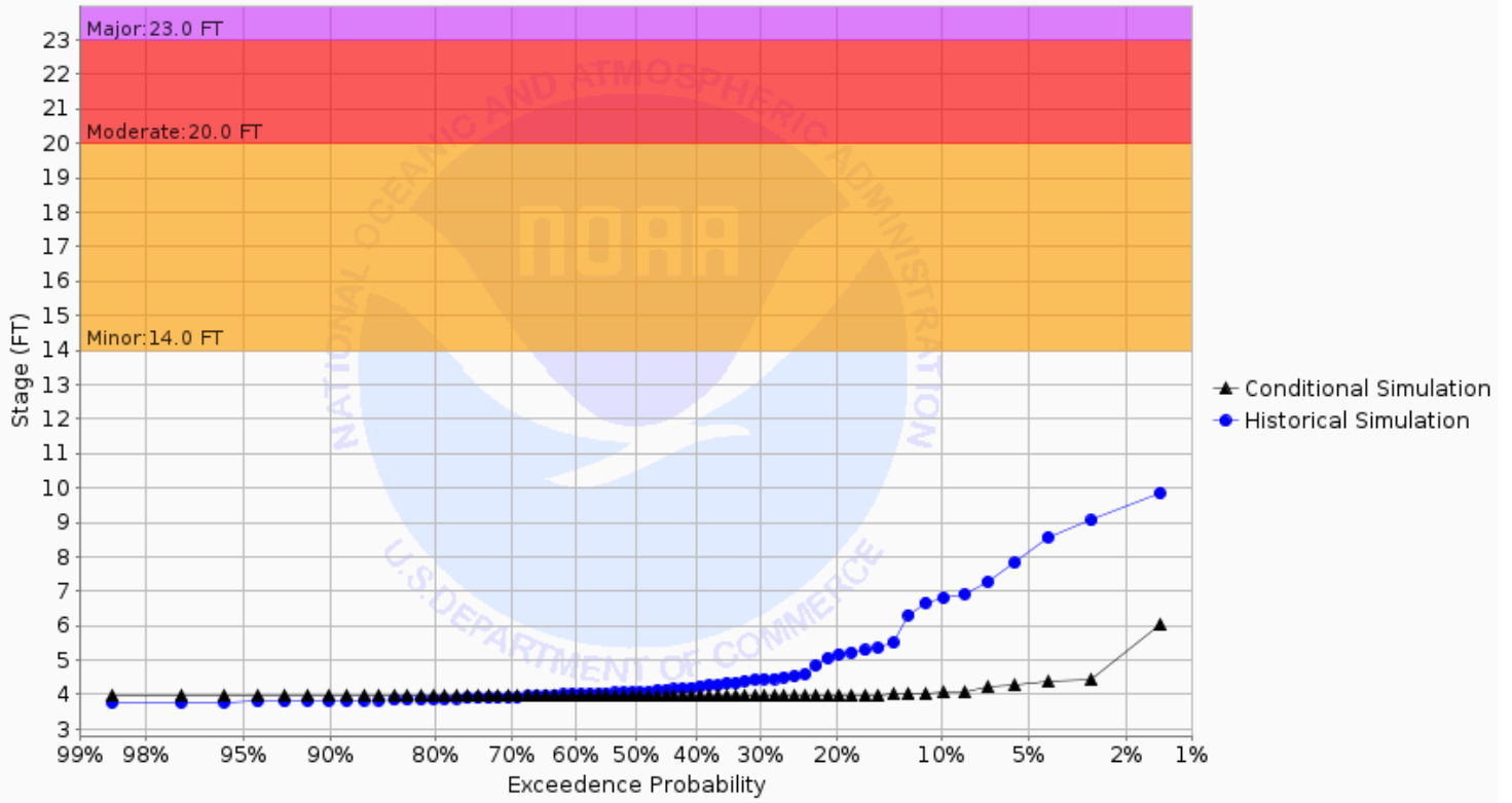
Chance of Exceeding River Stage at Marsh River at Shelly 4SE (SHYM5) Forecast for the period 10/28/2024 - 01/26/2025 This is a conditional simulation based on the conditions as of 10/21/2024
