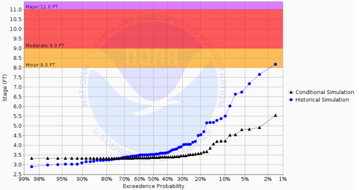
Chance of Exceeding River Stage at Buffalo River at Hawley 2SW (HWYM5) Forecast for the period 10/28/2024 - 01/26/2025 This is a conditional simulation based on the conditions as of 10/21/2024
