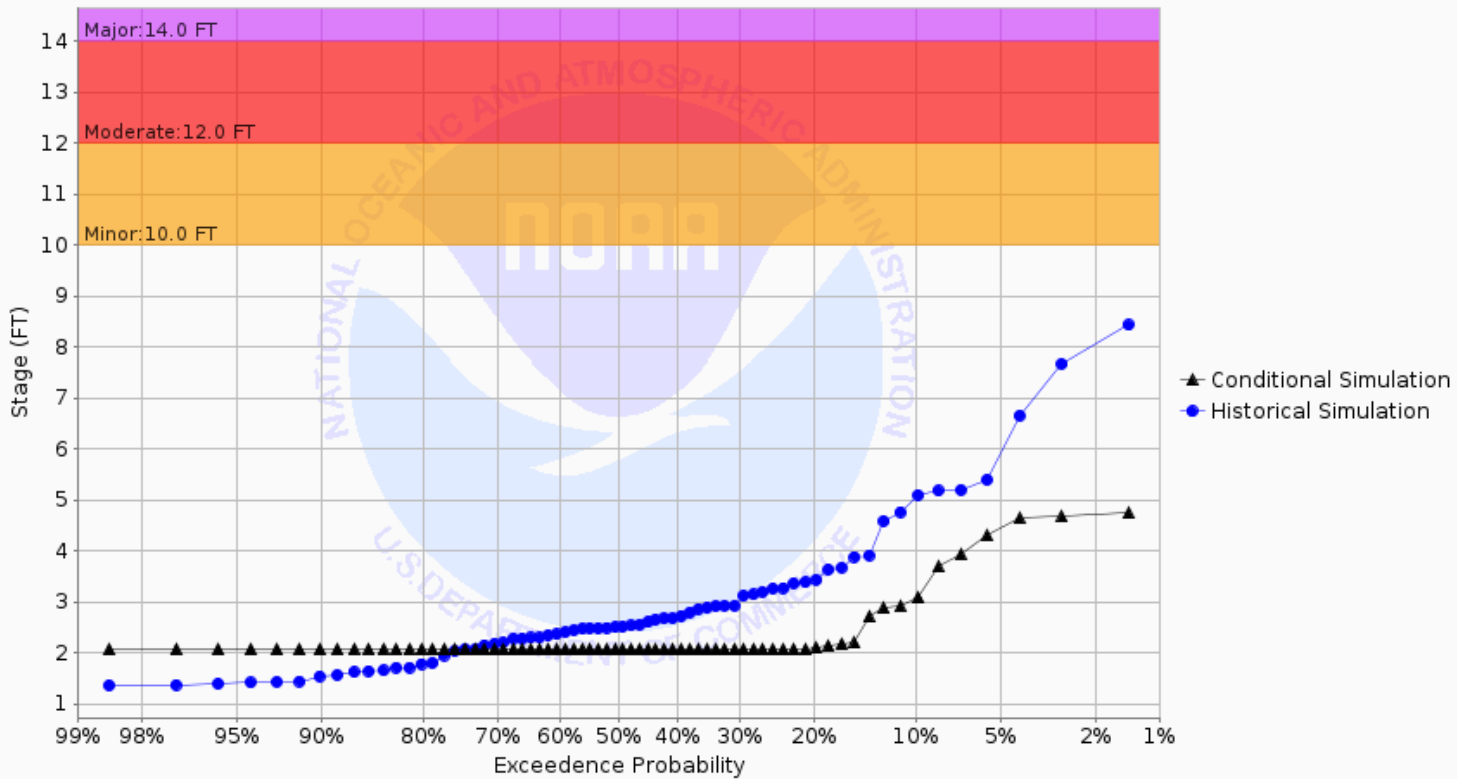
Chance of Exceeding River Stage at Wild Rice River at Twin Valley 1NE (TWVM5) Forecast for the period 10/28/2024 - 01/26/2025 This is a conditional simulation based on the conditions as of 10/21/2024
