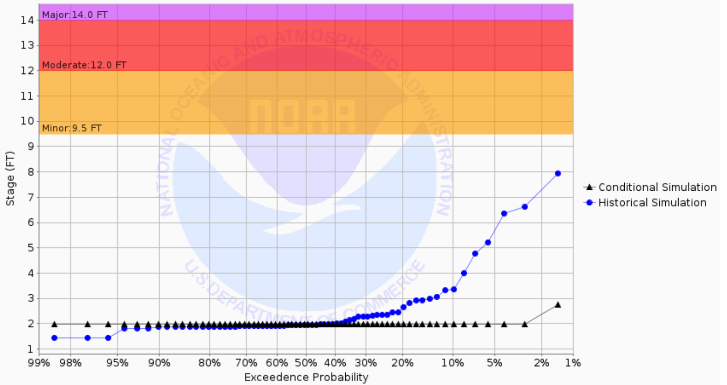
Chance of Exceeding River Stage at Maple River at Enderlin 1E (ENDN8) Forecast for the period 10/28/2024 - 01/26/2025 This is a conditional simulation based on the conditions as of 10/21/2024
