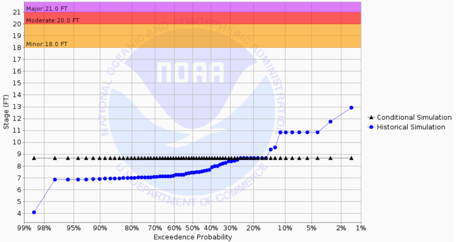
Chance of Exceeding River Stage at Sheyenne River Diversion at West Fargo (WFON8) Forecast for the period 10/28/2024 - 01/26/2025 This is a conditional simulation based on the conditions as of 10/21/2024
