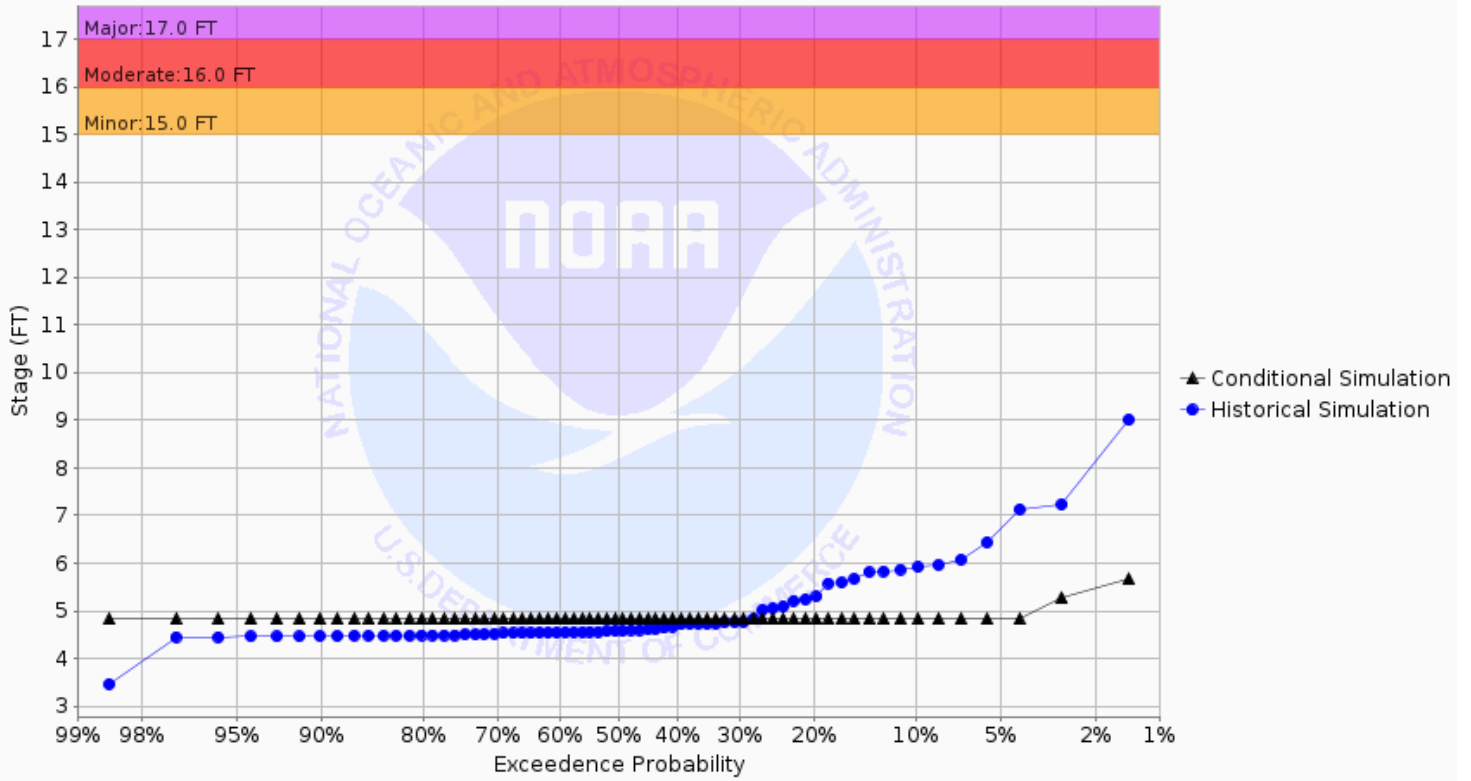
Chance of Exceeding River Stage at Sheyenne River at Valley City (VCRN8) Forecast for the period 10/28/2024 - 01/26/2025 This is a conditional simulation based on the conditions as of 10/21/2024
