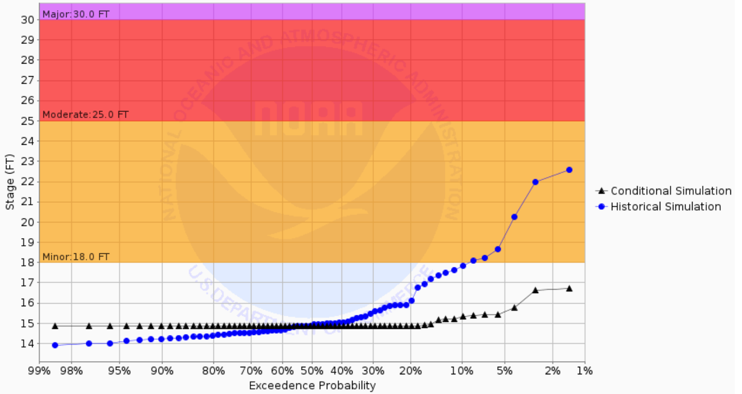
Chance of Exceeding River Stage at Red River of the North at Fargo WTP (FGON8) Forecast for the period 10/28/2024 - 01/26/2025 This is a conditional simulation based on the conditions as of 10/21/2024
