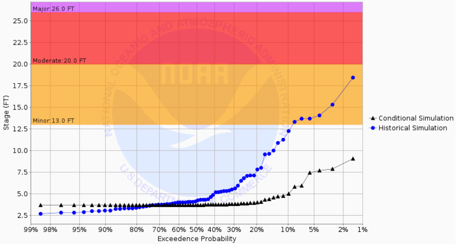
Chance of Exceeding River Stage at Buffalo River at Dilworth 7NE (DILM5) Forecast for the period 10/28/2024 - 01/26/2025 This is a conditional simulation based on the conditions as of 10/21/2024
