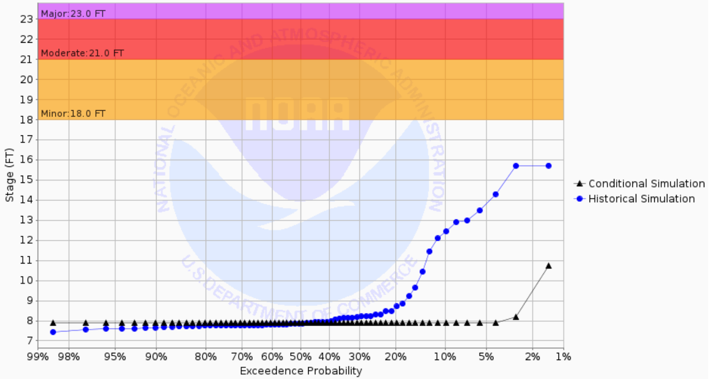
Chance of Exceeding River Stage at Maple River at Mapleton 3SW (MPLN8) Forecast for the period 10/28/2024 - 01/26/2025 This is a conditional simulation based on the conditions as of 10/21/2024
