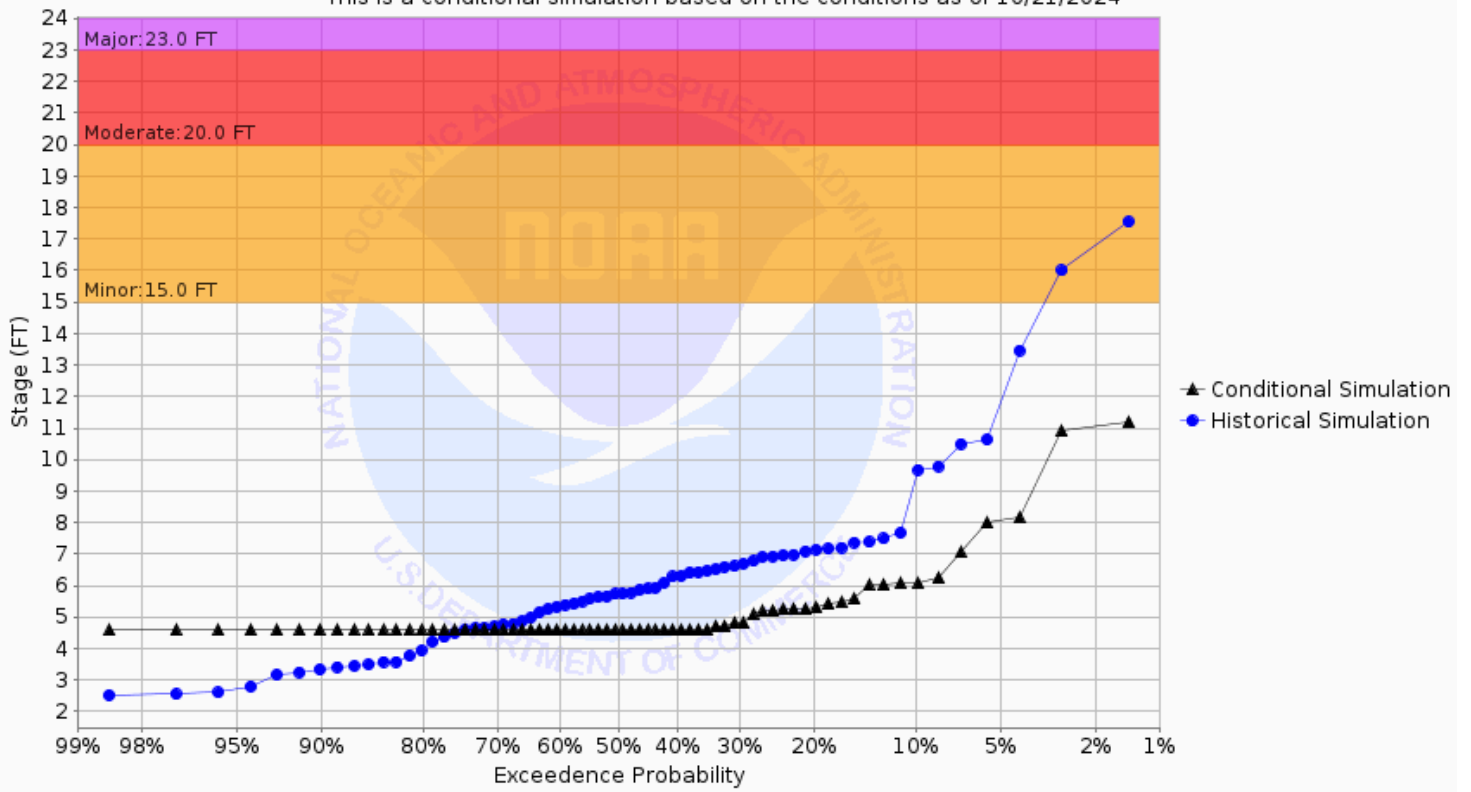
Chance of Exceeding River Stage at Snake River at Warren 3ENE-Morkassel Brdg (MKLM5) Forecast for the period 10/28/2024 - 01/26/2025 This is a conditional simulation based on the conditions as of 10/21/2024
