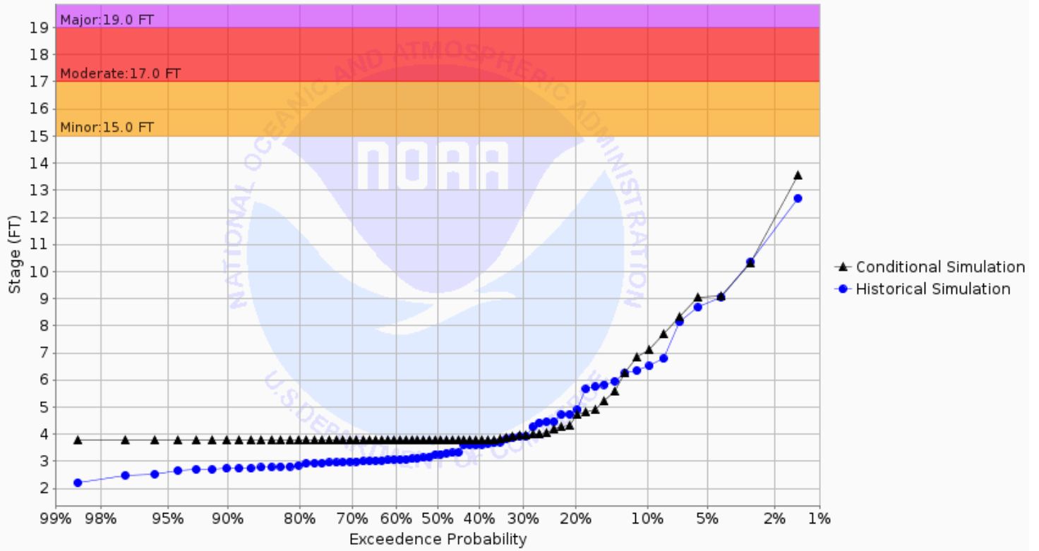
Chance of Exceeding River Stage at Sheyenne River at Lisbon (LBNN8) Forecast for the period 09/30/2024 - 12/29/2024 This is a conditional simulation based on the conditions as of 09/23/2024
