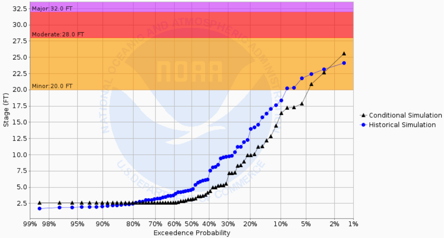
Chance of Exceeding River Stage at Wild Rice River at Hendrum (HNDM5) Forecast for the period 09/30/2024 - 12/29/2024 This is a conditional simulation based on the conditions as of 09/23/2024
