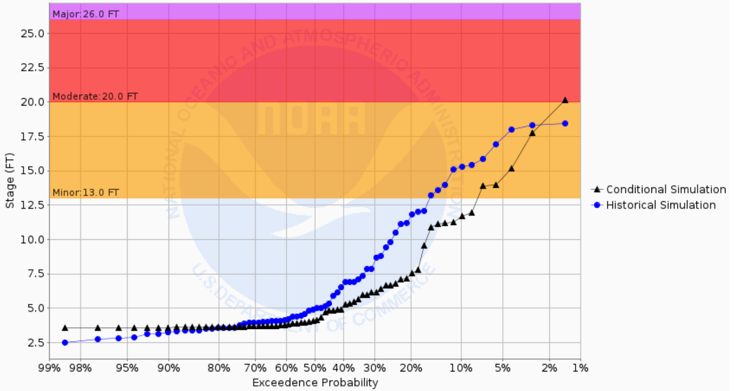
Chance of Exceeding River Stage at Buffalo River at Dilworth 7NE (DILM5) Forecast for the period 09/30/2024 - 12/29/2024 This is a conditional simulation based on the conditions as of 09/23/2024
