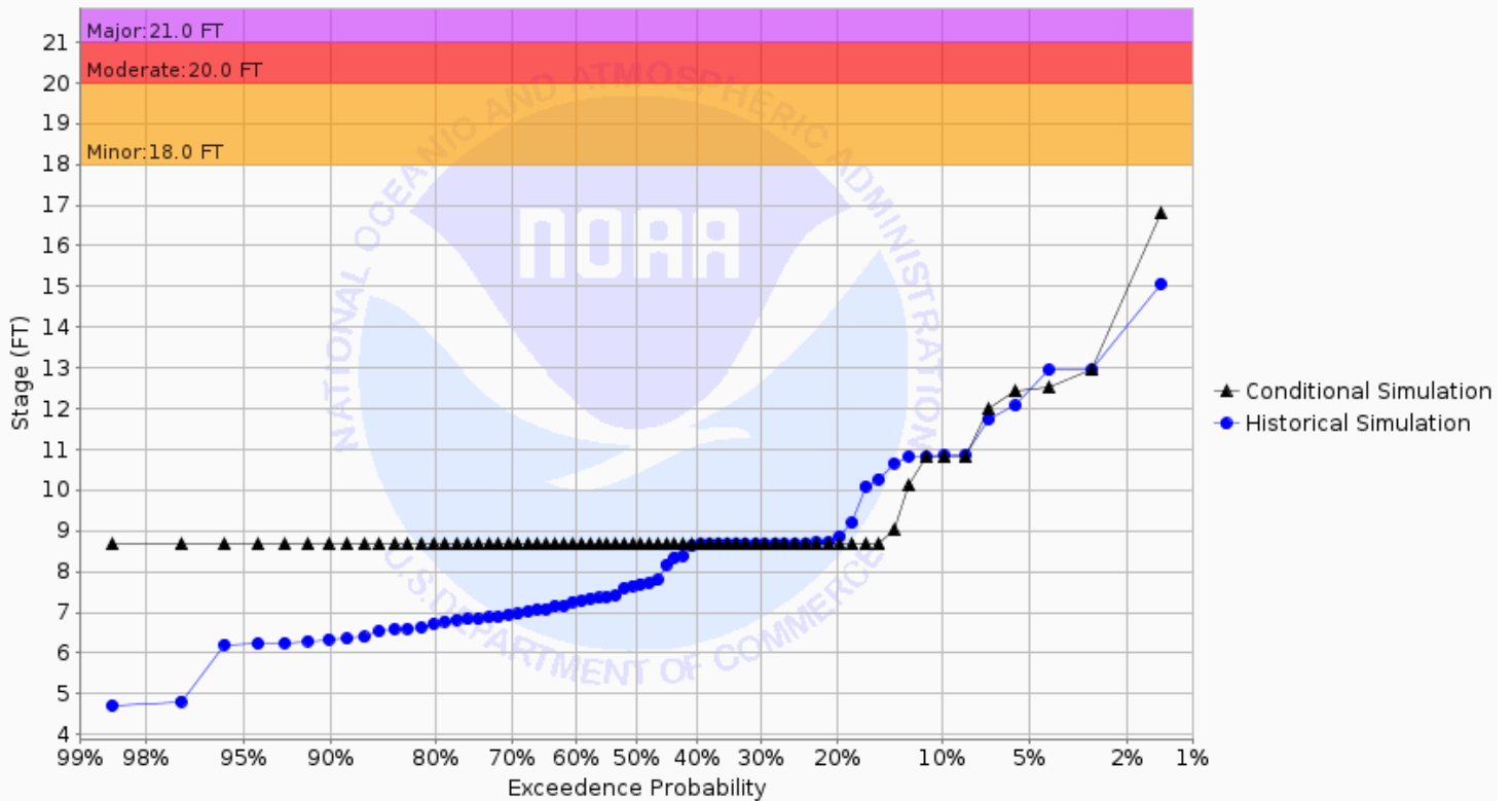
Chance of Exceeding River Stage at Sheyenne River Diversion at West Fargo (WFON8) Forecast for the period 09/30/2024 - 12/29/2024 This is a conditional simulation based on the conditions as of 09/23/2024
