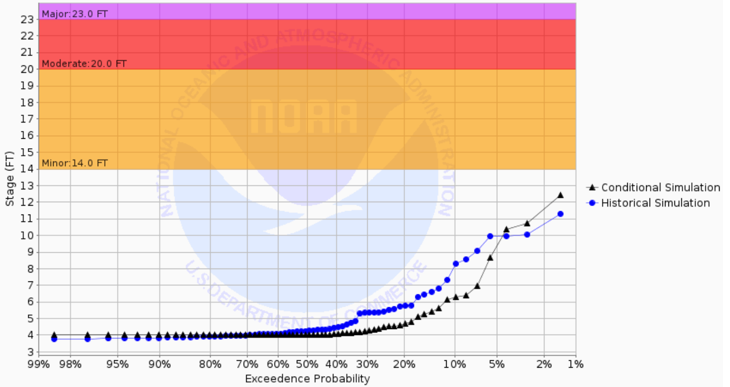
Chance of Exceeding River Stage at Marsh River at Shelly 4SE (SHYM5) Forecast for the period 09/30/2024 - 12/29/2024 This is a conditional simulation based on the conditions as of 09/23/2024
