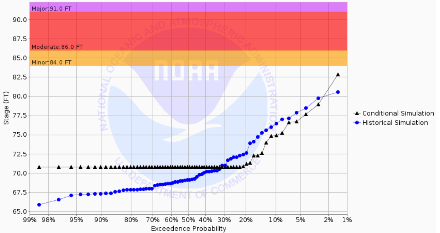
Chance of Exceeding River Stage at Sheyenne River at Harwood (HWDN8) Forecast for the period 09/30/2024 - 12/29/2024 This is a conditional simulation based on the conditions as of 09/23/2024
