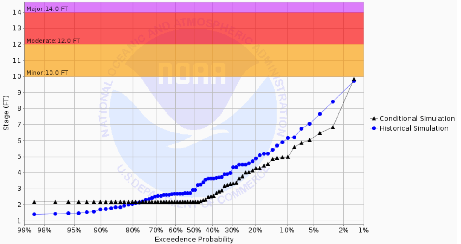
Chance of Exceeding River Stage at Wild Rice River at Twin Valley 1NE (TWVM5) Forecast for the period 09/30/2024 - 12/29/2024 This is a conditional simulation based on the conditions as of 09/23/2024
