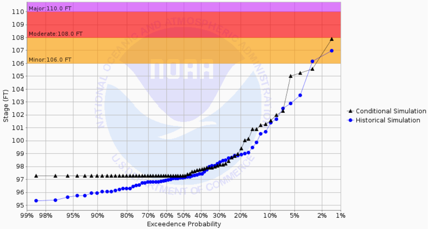
Chance of Exceeding River Stage at Snake River at Alvarado (ALVM5) Forecast for the period 09/30/2024 - 12/29/2024 This is a conditional simulation based on the conditions as of 09/23/2024
