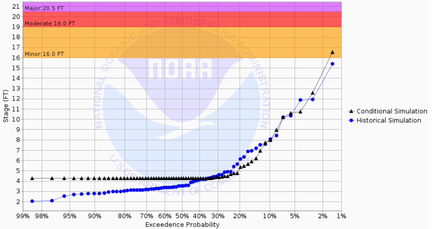
Chance of Exceeding River Stage at Sheyenne River at Kindred 2SE (KNDN8) Forecast for the period 09/30/2024 - 12/29/2024 This is a conditional simulation based on the conditions as of 09/23/2024
