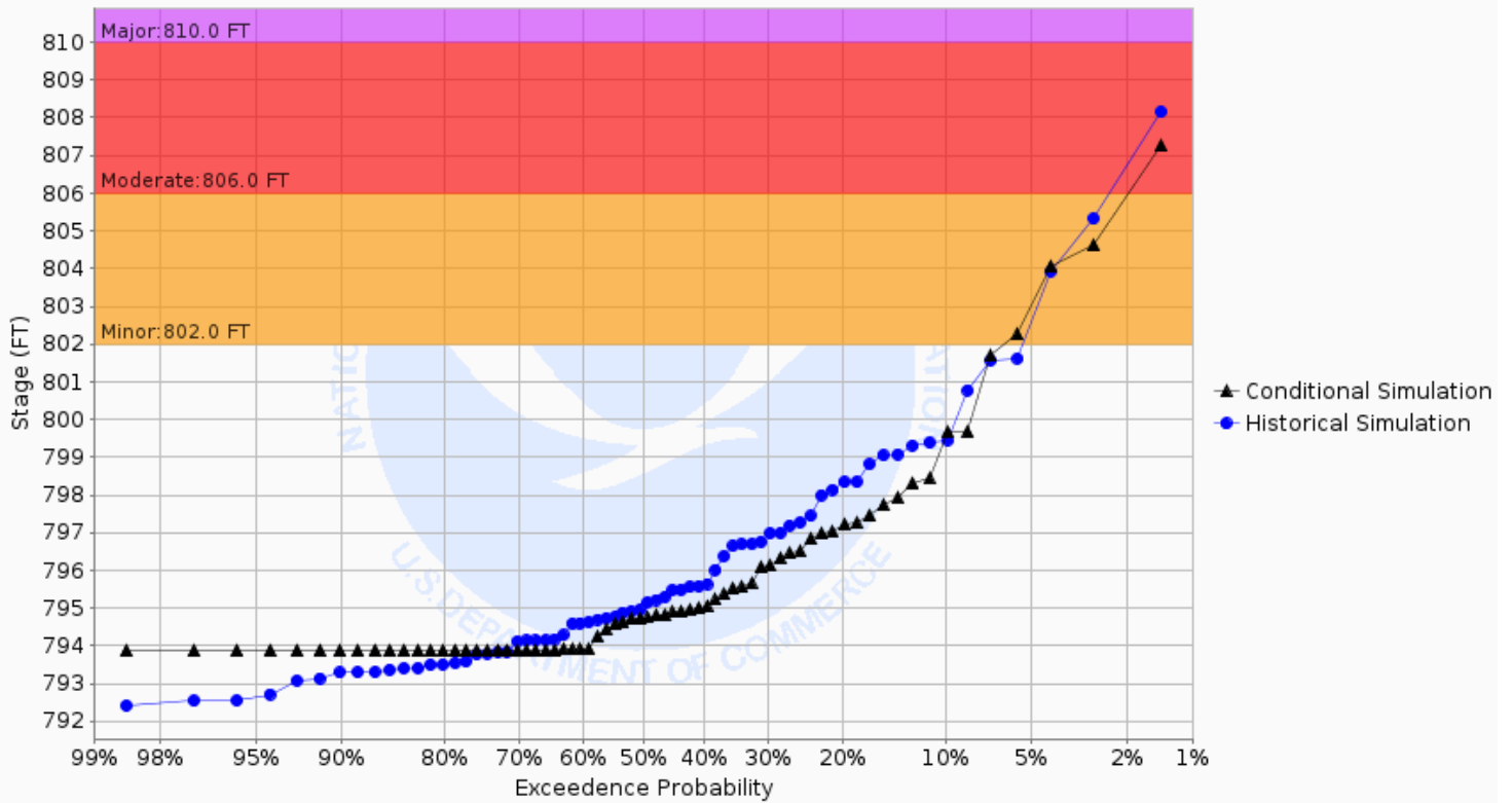
Chance of Exceeding River Stage at Two Rivers River at Hallock (HLLM5) Forecast for the period 09/30/2024 - 12/29/2024 This is a conditional simulation based on the conditions as of 09/23/2024
