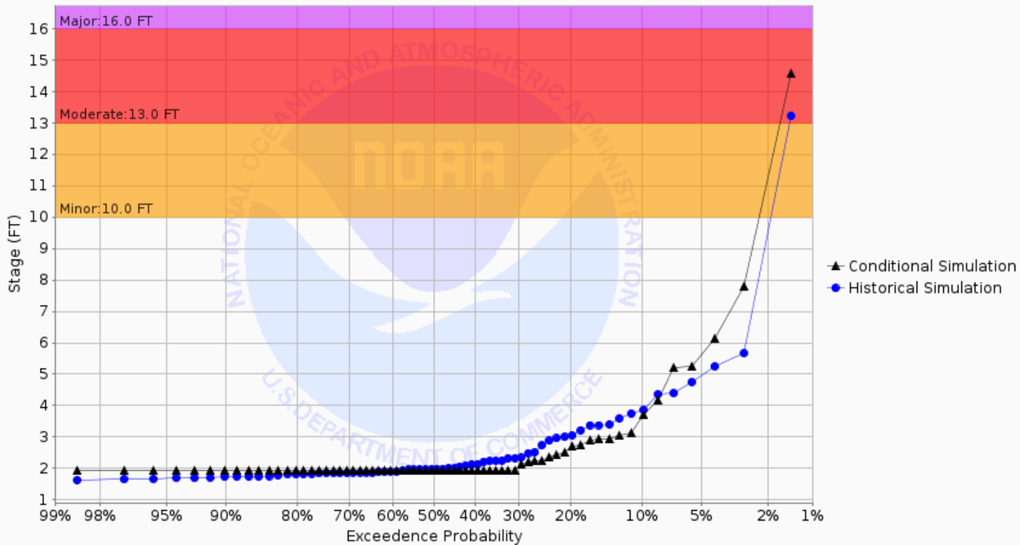
Chance of Exceeding River Stage at Goose River at Hillsboro (HGRN8) Forecast for the period 09/30/2024 - 12/29/2024 This is a conditional simulation based on the conditions as of 09/23/2024
