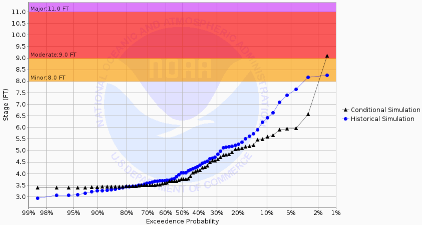
Chance of Exceeding River Stage at Buffalo River at Hawley 2SW (HWYM5) Forecast for the period 09/30/2024 - 12/29/2024 This is a conditional simulation based on the conditions as of 09/23/2024
