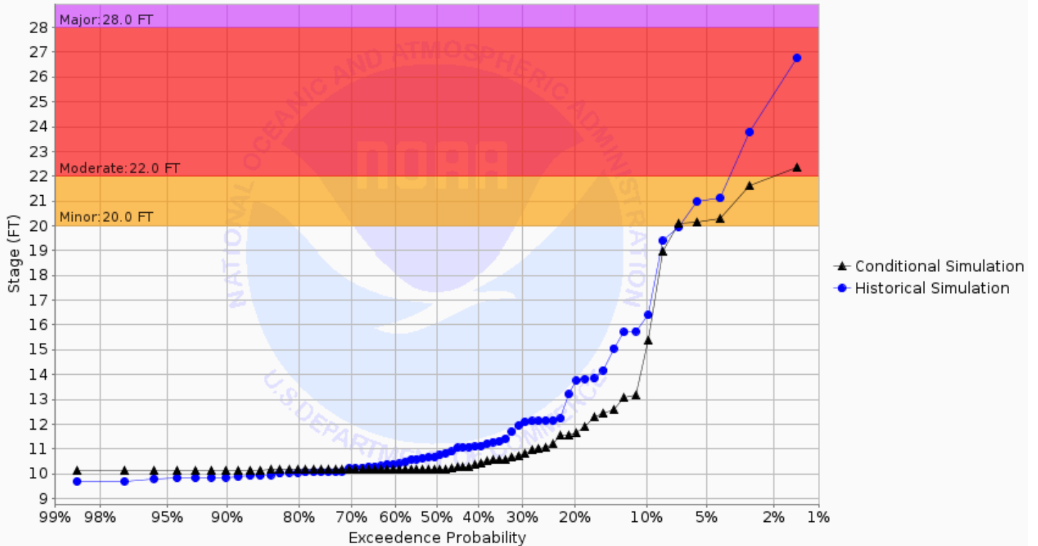
Chance of Exceeding River Stage at Wild Rice River at Abercrombie 2WNW (ABRN8) Forecast for the period 09/30/2024 - 12/29/2024 This is a conditional simulation based on the conditions as of 09/23/2024
