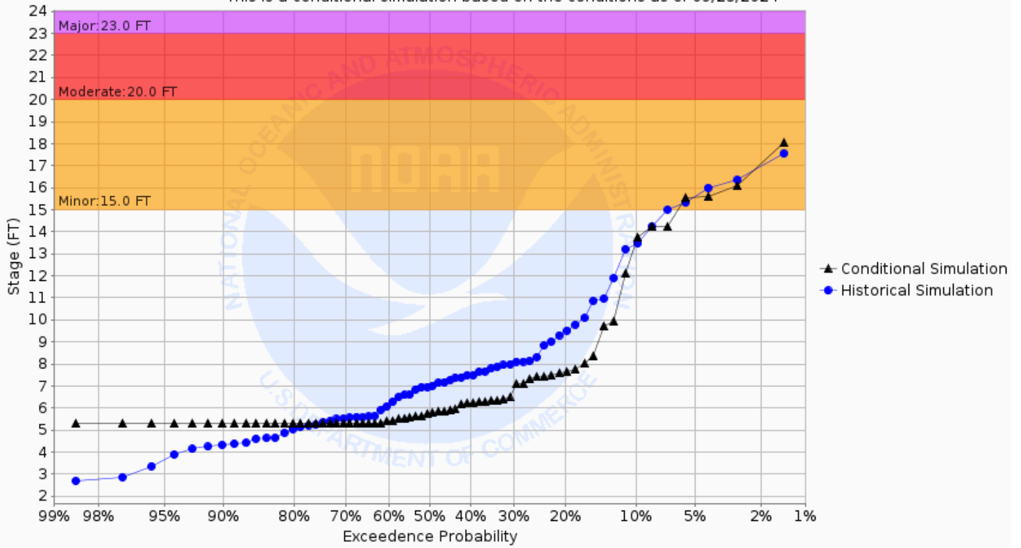
Chance of Exceeding River Stage at Red Lake River at Crookston (CRKM5) Forecast for the period 09/30/2024 - 12/29/2024 This is a conditional simulation based on the conditions as of 09/23/2024
