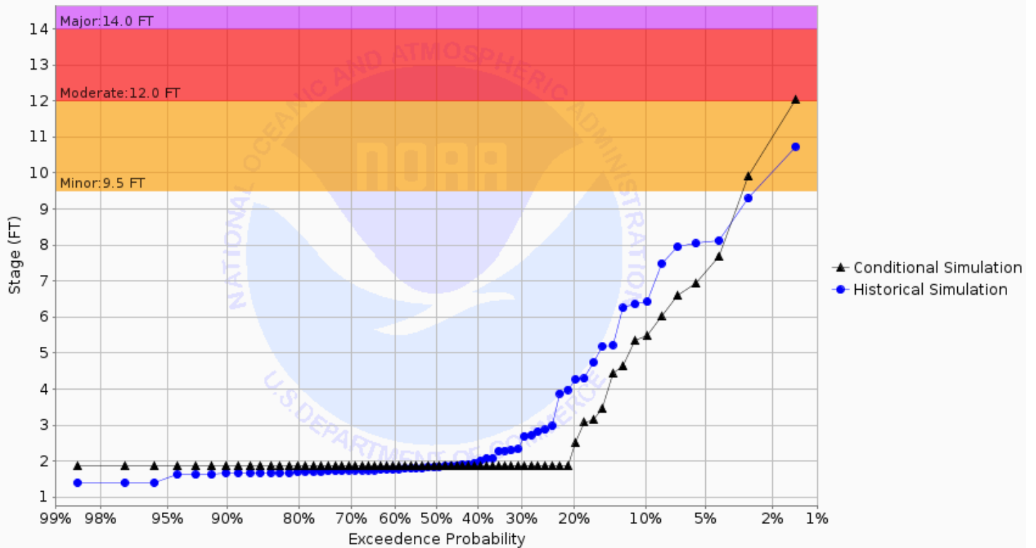
Chance of Exceeding River Stage at Maple River at Enderlin 1E (ENDN8) Forecast for the period 09/30/2024 - 12/29/2024 This is a conditional simulation based on the conditions as of 09/23/2024
