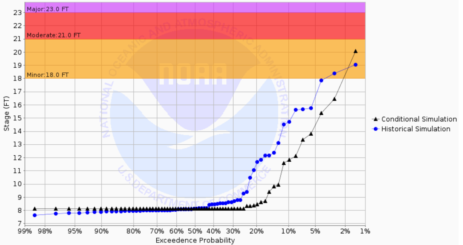
Chance of Exceeding River Stage at Maple River at Mapleton 3SW (MPLN8) Forecast for the period 09/30/2024 - 12/29/2024 This is a conditional simulation based on the conditions as of 09/23/2024
