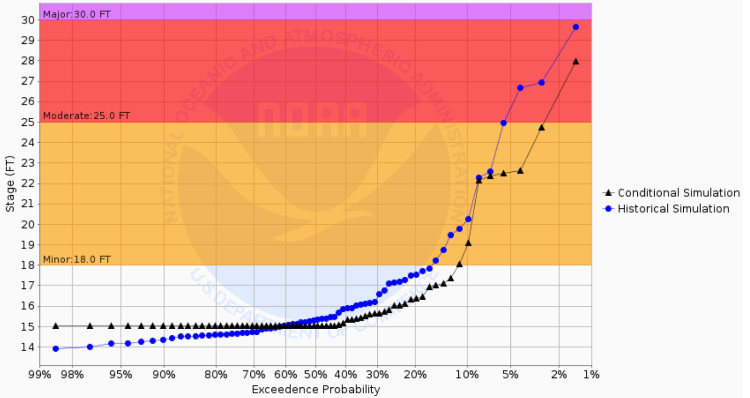
Chance of Exceeding River Stage at Red River of the North at Fargo WTP (FGON8) Forecast for the period 09/30/2024 - 12/29/2024 This is a conditional simulation based on the conditions as of 09/23/2024
