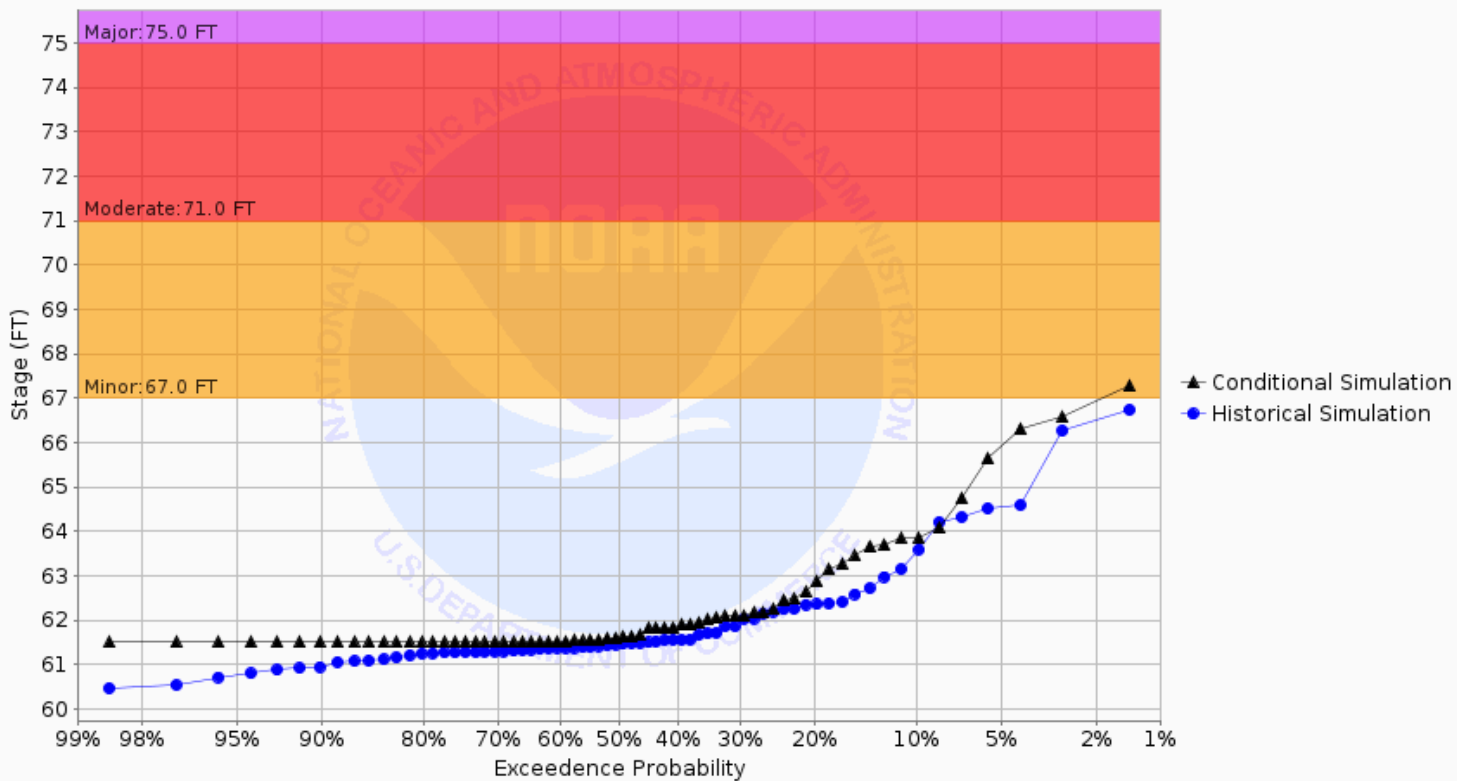
Chance of Exceeding River Stage at Snake River at Warren 3ENE-Morkassel Brdg (MKLM5) Forecast for the period 09/30/2024 - 12/29/2024 This is a conditional simulation based on the conditions as of 09/23/2024
