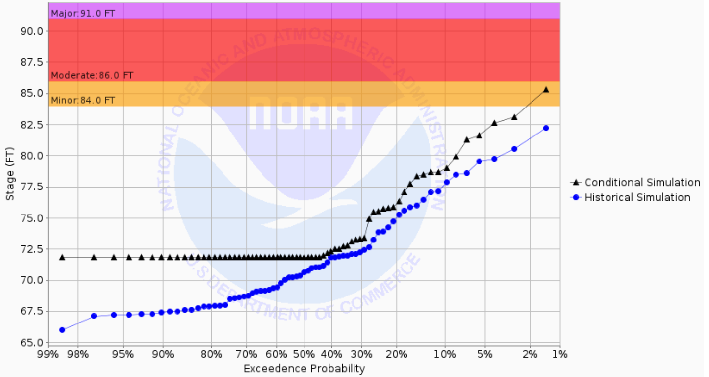
Chance of Exceeding River Stage at Sheyenne River at Harwood (HWDN8) Forecast for the period 08/26/2024 - 11/24/2024 This is a conditional simulation based on the conditions as of 08/19/2024
