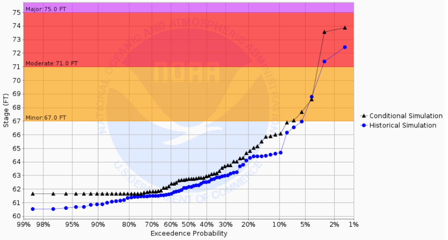
Chance of Exceeding River Stage at Snake River at Warren 3ENE-Morkassel Brdg (MKLM5) Forecast for the period 08/26/2024 - 11/24/2024 This is a conditional simulation based on the conditions as of 08/19/2024
