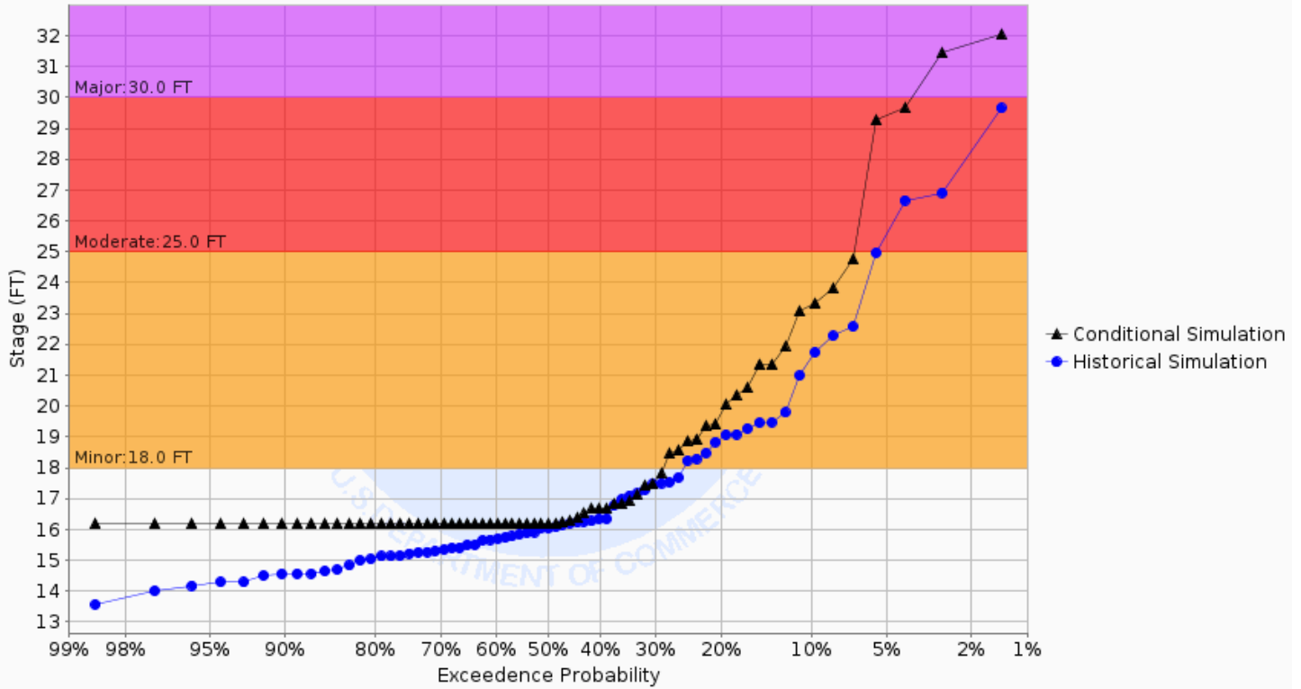
Chance of Exceeding River Stage at Red River of the North at Fargo WTP (FGON8) Forecast for the period 08/26/2024 - 11/24/2024 This is a conditional simulation based on the conditions as of 08/19/2024
