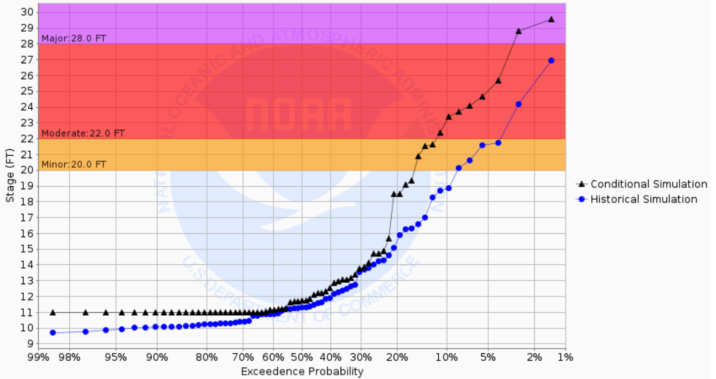
Chance of Exceeding River Stage at Wild Rice River at Abercrombie 2WNW (ABRN8) Forecast for the period 08/26/2024 - 11/24/2024 This is a conditional simulation based on the conditions as of 08/19/2024
