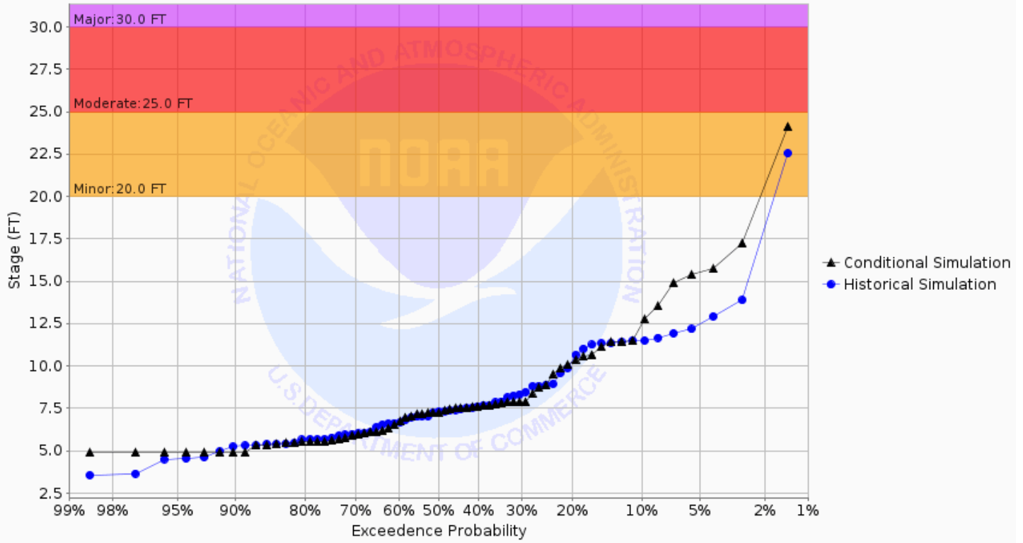
Chance of Exceeding River Stage at Sand Hill River at Climax (CLXM5) Forecast for the period 08/26/2024 - 11/24/2024 This is a conditional simulation based on the conditions as of 08/19/2024
