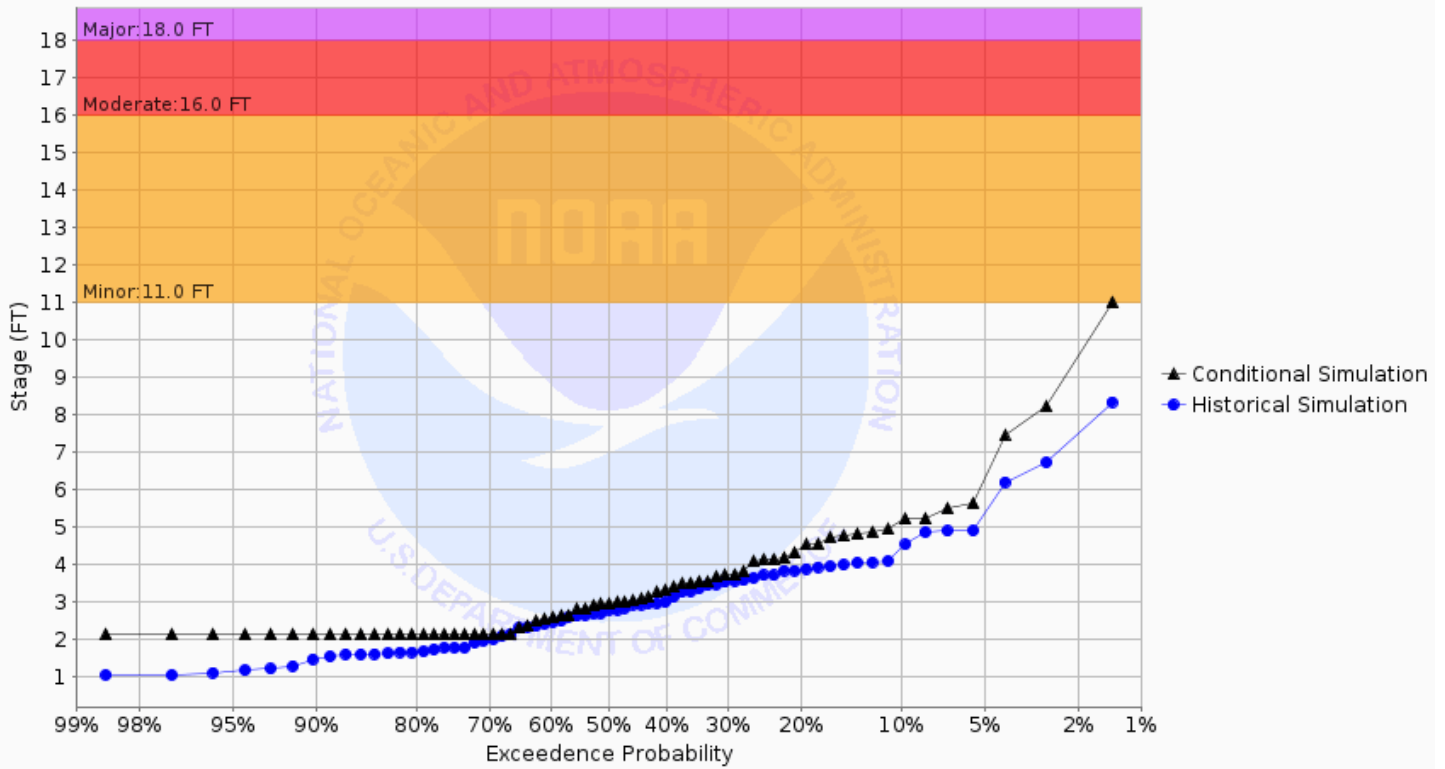
Chance of Exceeding River Stage at Pembina River at Walhalla (WLHN8) Forecast for the period 08/26/2024 - 11/24/2024 This is a conditional simulation based on the conditions as of 08/19/2024
