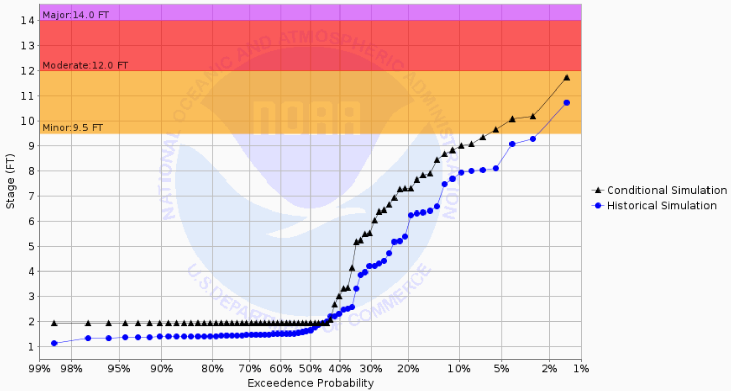
Chance of Exceeding River Stage at Maple River at Enderlin 1E (ENDN8) Forecast for the period 08/26/2024 - 11/24/2024 This is a conditional simulation based on the conditions as of 08/19/2024
