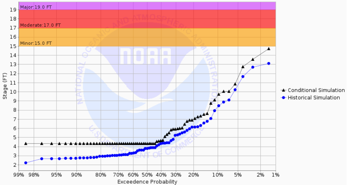
Chance of Exceeding River Stage at Sheyenne River at Lisbon (LBNN8) Forecast for the period 08/26/2024 - 11/24/2024 This is a conditional simulation based on the conditions as of 08/19/2024
