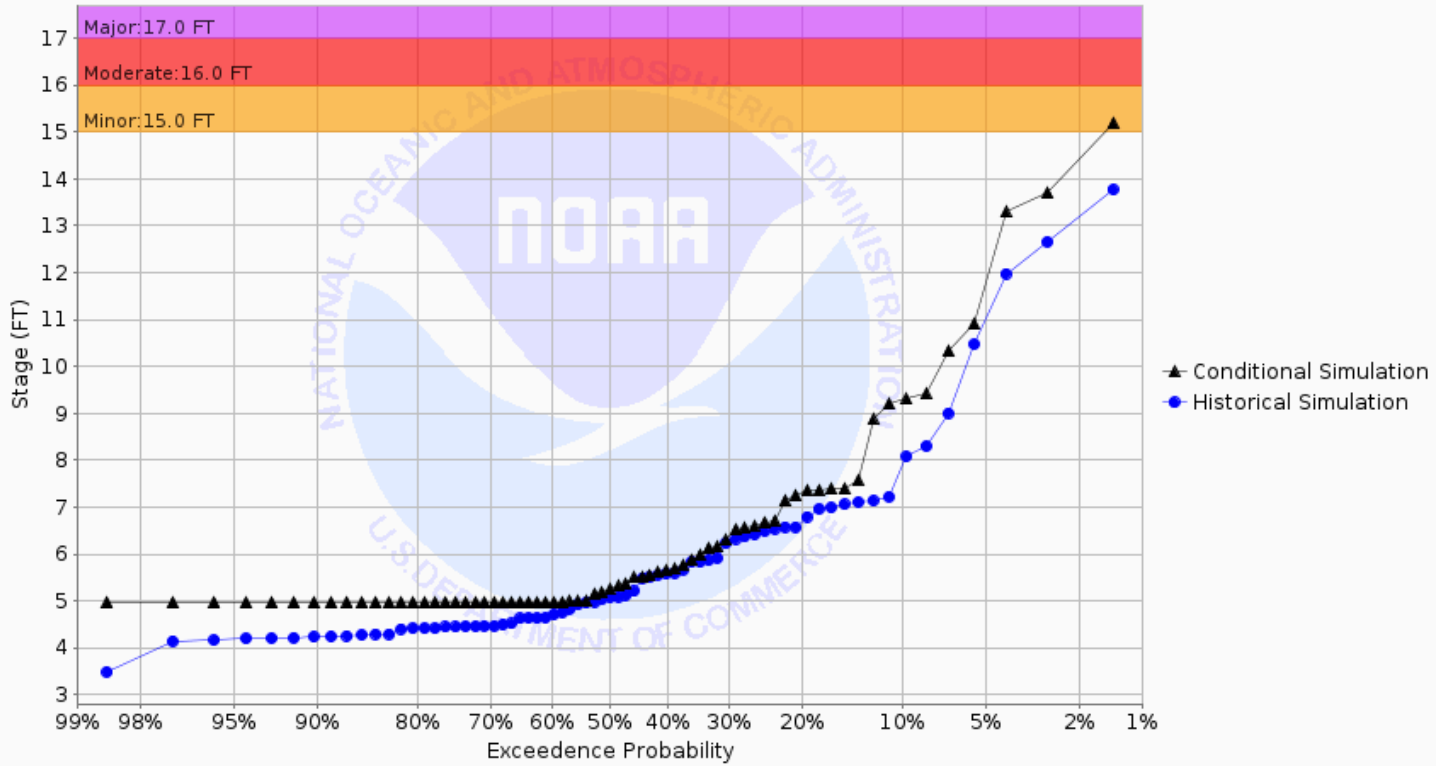
Chance of Exceeding River Stage at Sheyenne River at Valley City (VCRN8) Forecast for the period 08/26/2024 - 11/24/2024 This is a conditional simulation based on the conditions as of 08/19/2024
