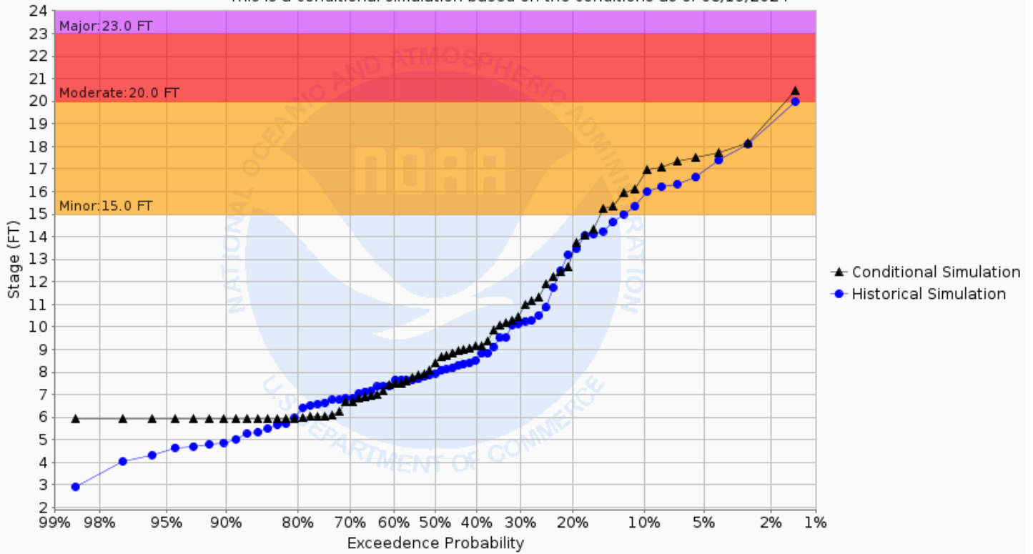
Chance of Exceeding River Stage at Red Lake River at Crookston (CRKM5) Forecast for the period 08/26/2024 - 11/24/2024 This is a conditional simulation based on the conditions as of 08/19/2024
