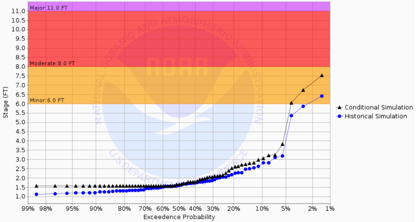
Chance of Exceeding River Stage at Forest River at Minto (MTON8) Forecast for the period 08/26/2024 - 11/24/2024 This is a conditional simulation based on the conditions as of 08/19/2024
