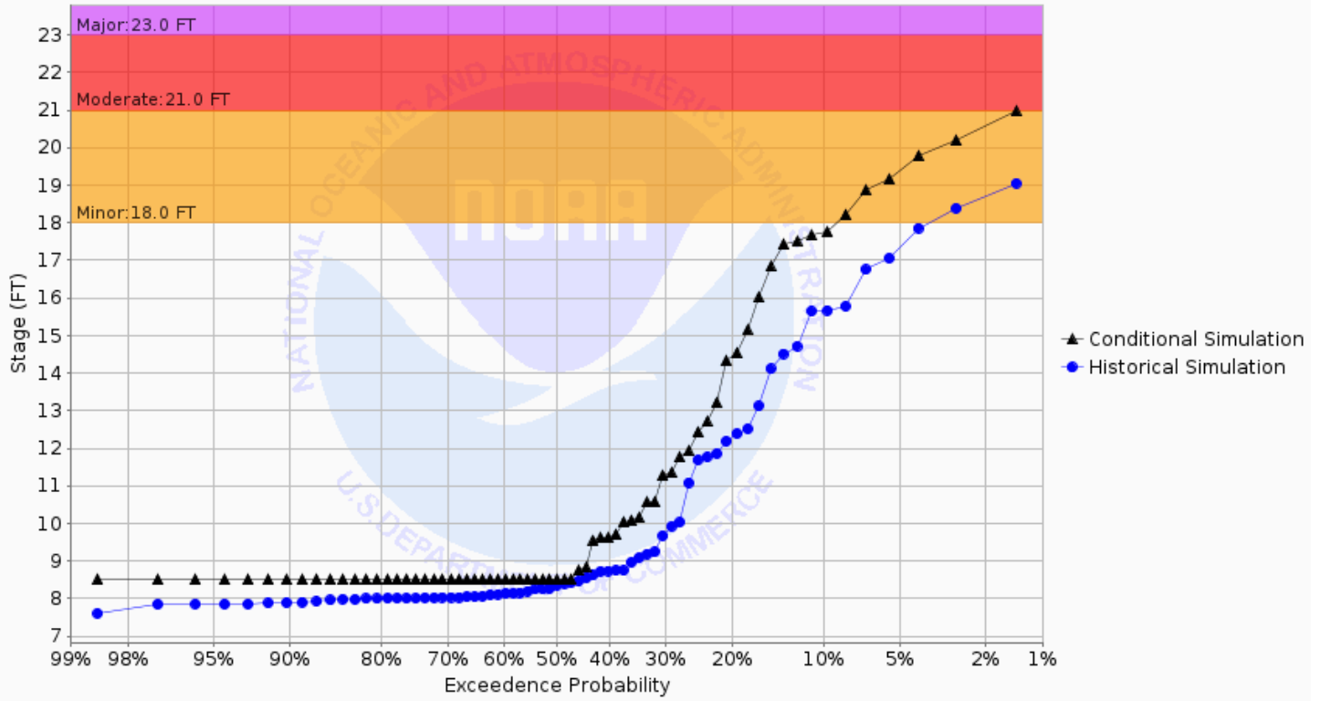
Chance of Exceeding River Stage at Maple River at Mapleton 3SW (MPLN8) Forecast for the period 08/26/2024 - 11/24/2024 This is a conditional simulation based on the conditions as of 08/19/2024
