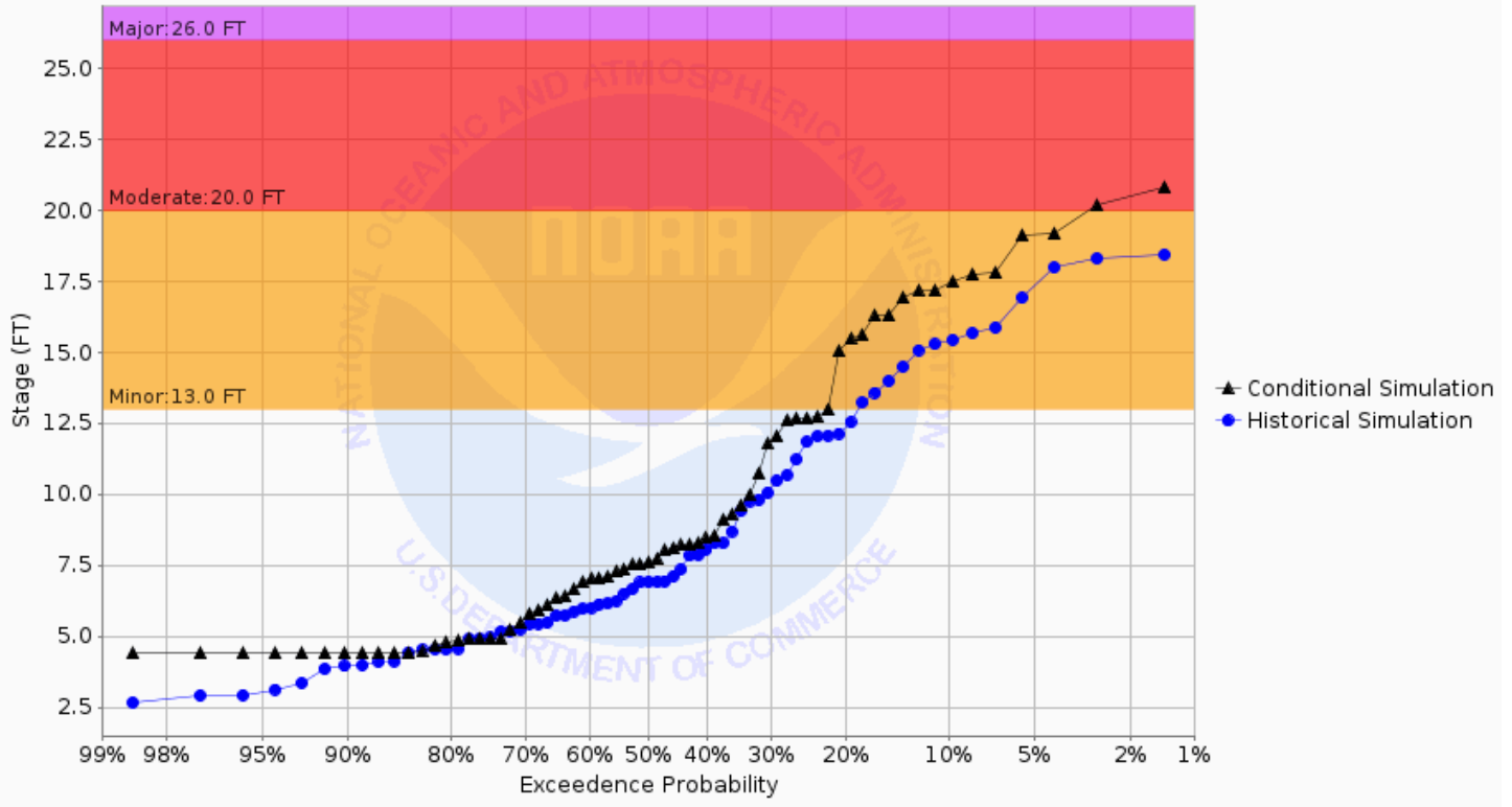
Chance of Exceeding River Stage at Buffalo River at Dilworth 7NE (DILM5) Forecast for the period 08/26/2024 - 11/24/2024 This is a conditional simulation based on the conditions as of 08/19/2024
