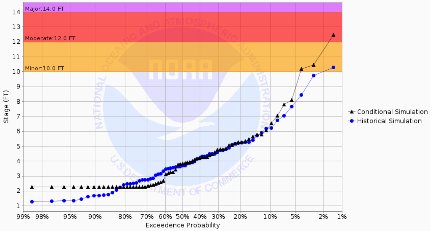
Chance of Exceeding River Stage at Wild Rice River at Twin Valley 1NE (TWVM5) Forecast for the period 08/26/2024 - 11/24/2024 This is a conditional simulation based on the conditions as of 08/19/2024
