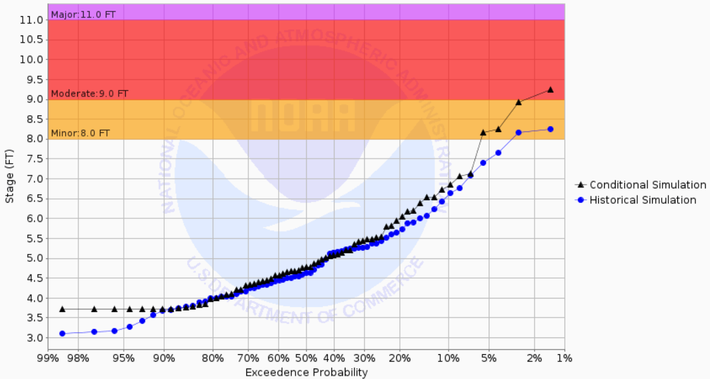
Chance of Exceeding River Stage at Buffalo River at Hawley 2SW (HWYM5) Forecast for the period 08/26/2024 - 11/24/2024 This is a conditional simulation based on the conditions as of 08/19/2024
