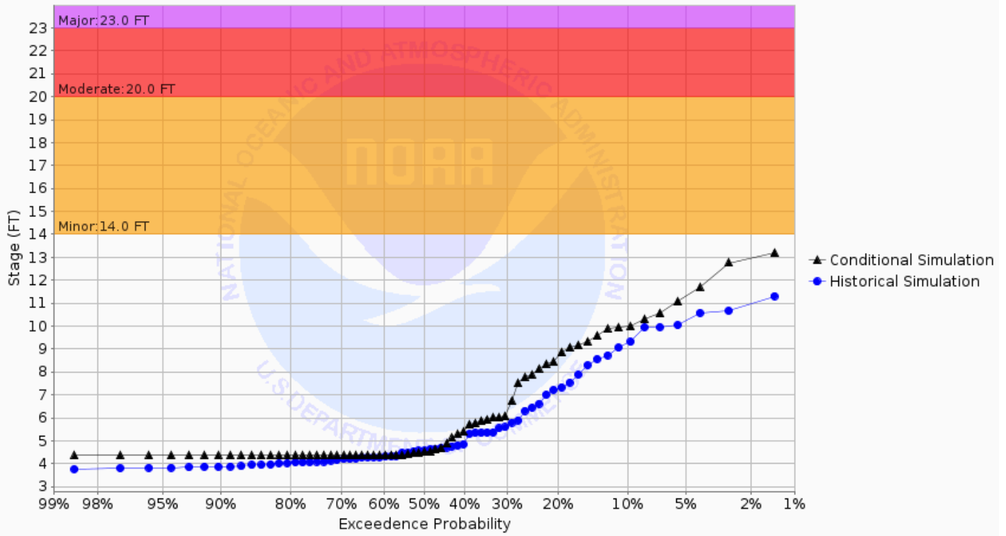
Chance of Exceeding River Stage at Marsh River at Shelly 4SE (SHYM5) Forecast for the period 08/26/2024 - 11/24/2024 This is a conditional simulation based on the conditions as of 08/19/2024
