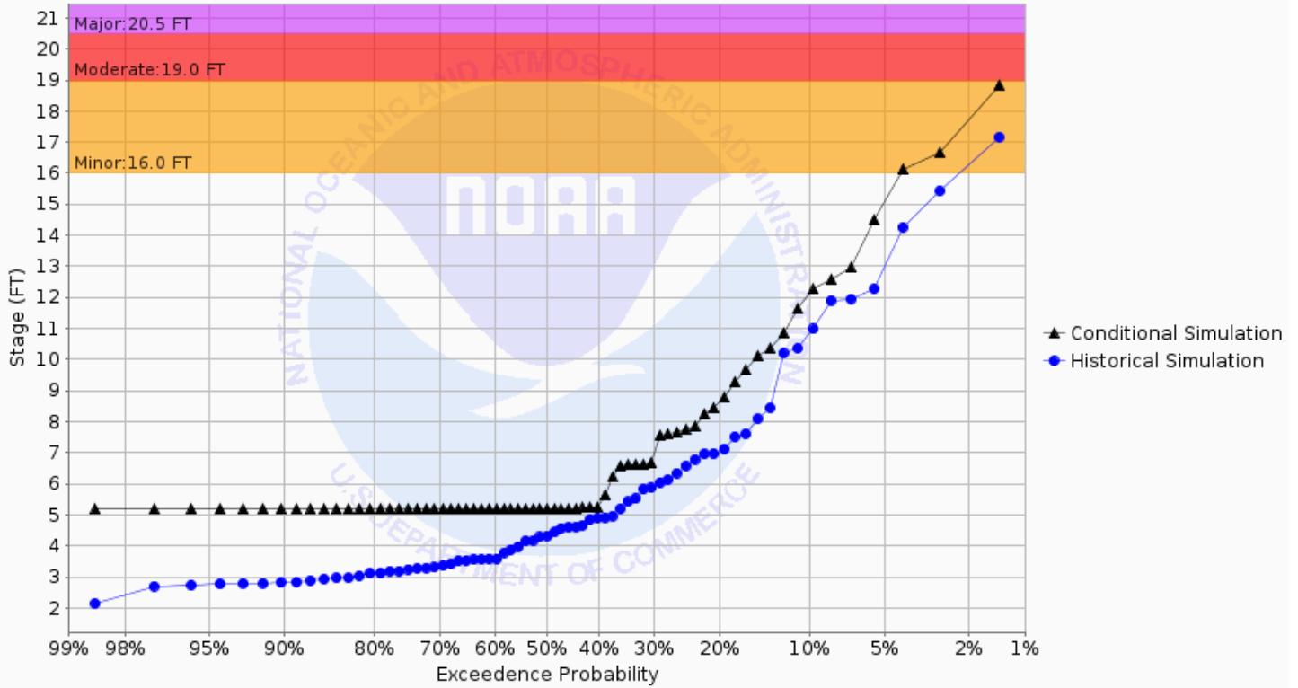
Chance of Exceeding River Stage at Sheyenne River at Kindred 2SE (KNDN8) Forecast for the period 08/26/2024 - 11/24/2024 This is a conditional simulation based on the conditions as of 08/19/2024
