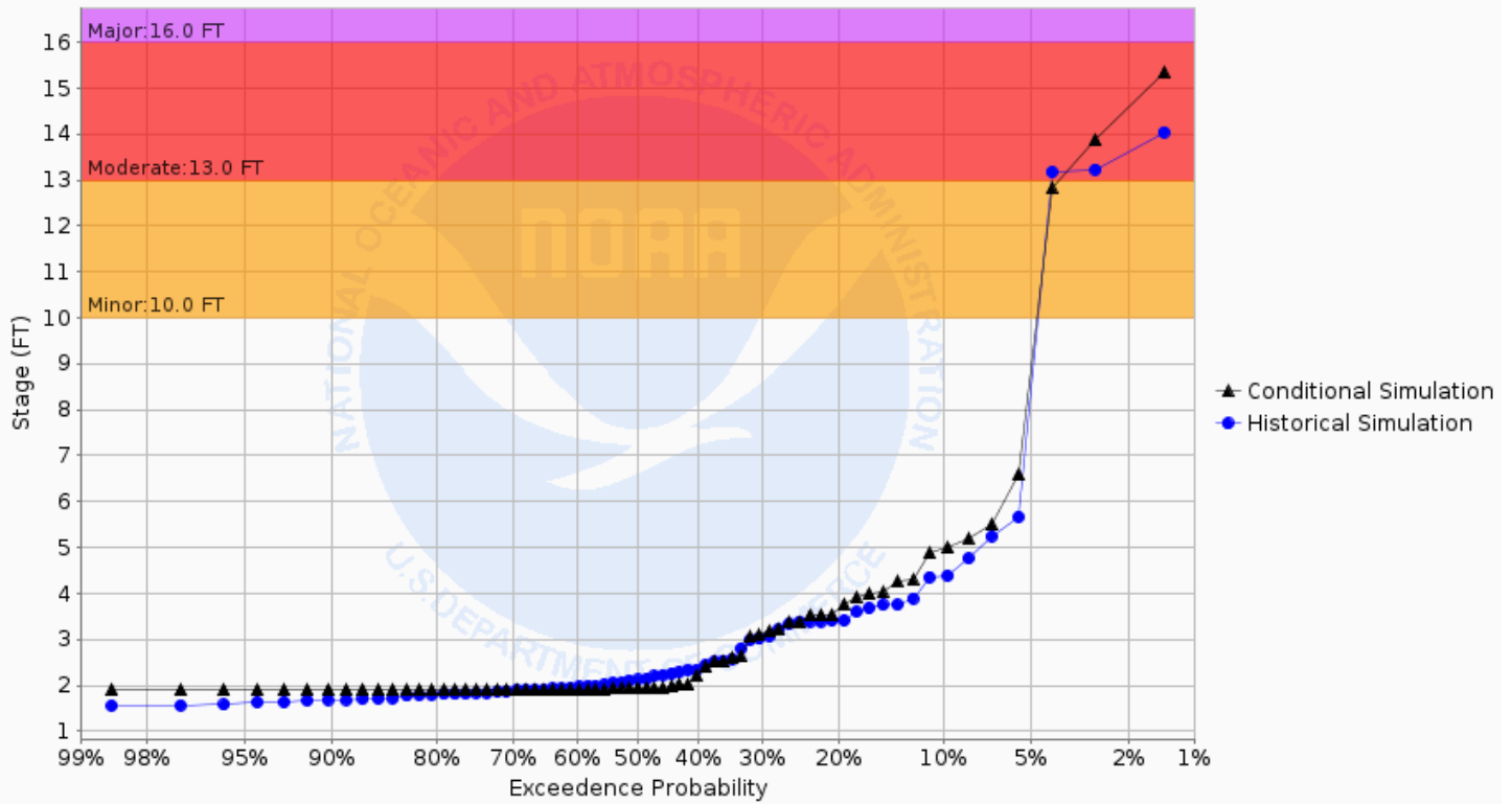
Chance of Exceeding River Stage at Goose River at Hillsboro (HGRN8) Forecast for the period 08/26/2024 - 11/24/2024 This is a conditional simulation based on the conditions as of 08/19/2024
