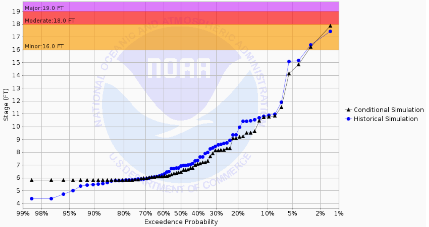
Chance of Exceeding River Stage at Roseau River at Roseau - Center St Brdg (ROSM5) Forecast for the period 08/26/2024 - 11/24/2024 This is a conditional simulation based on the conditions as of 08/19/2024
