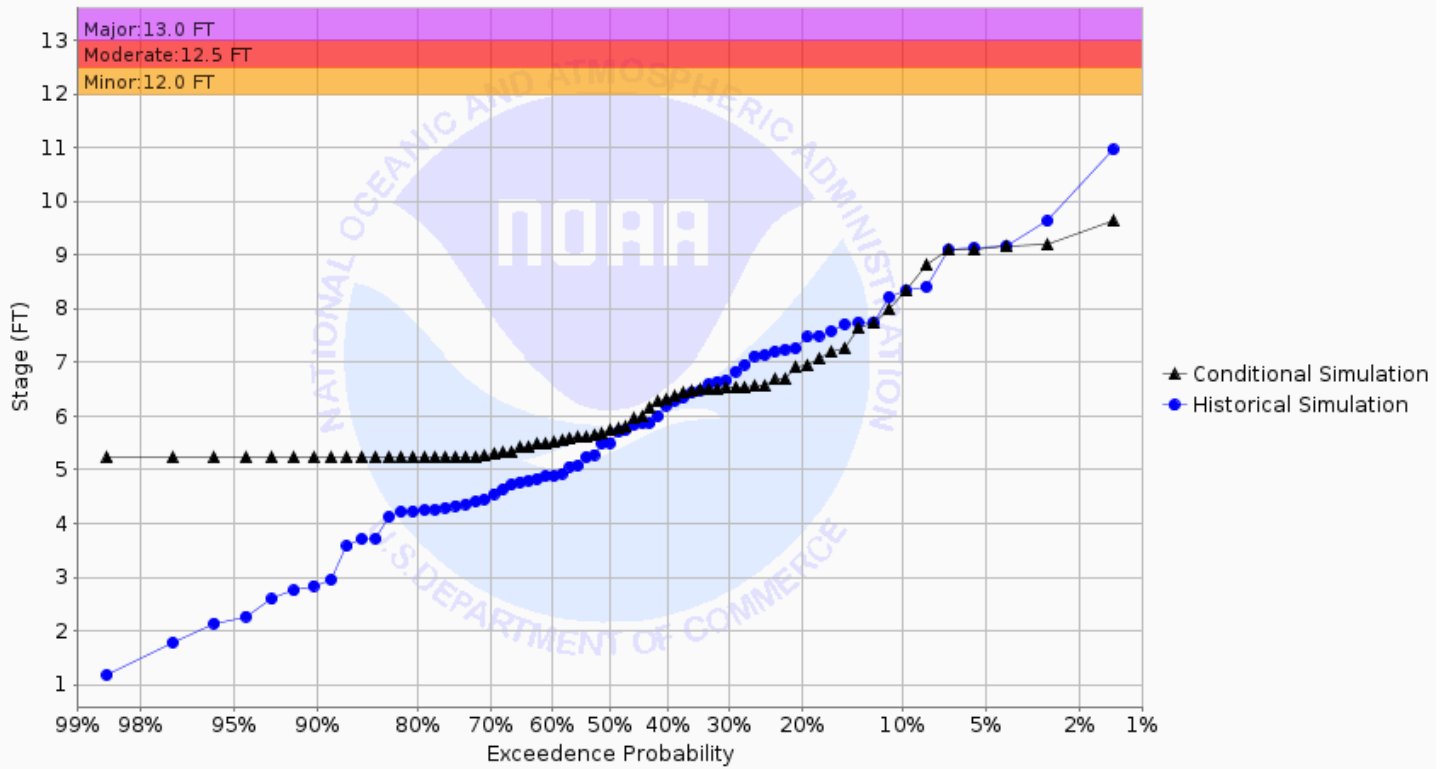
Chance of Exceeding River Stage at Red Lake River at High Landing (HIGM5) Forecast for the period 08/26/2024 - 11/24/2024 This is a conditional simulation based on the conditions as of 08/19/2024
