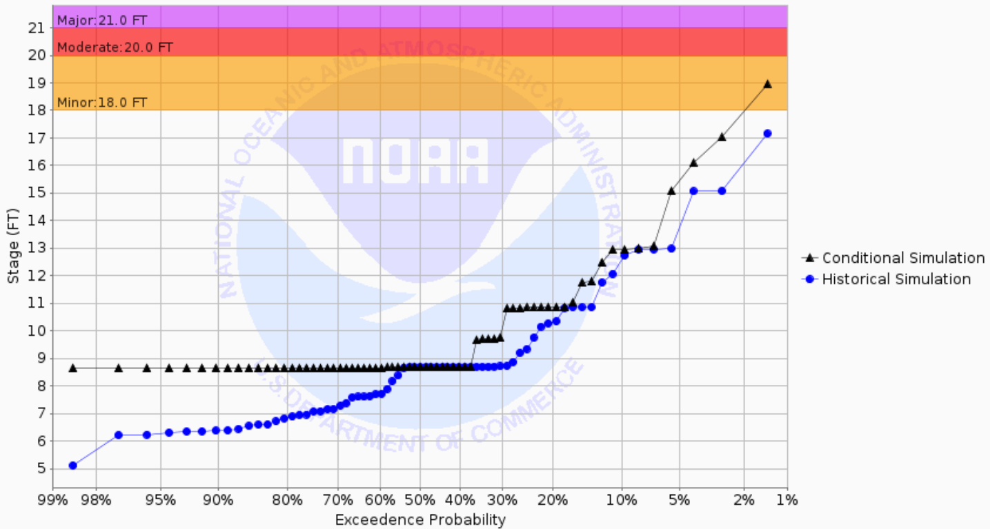
Chance of Exceeding River Stage at Sheyenne River Diversion at West Fargo (WFON8) Forecast for the period 08/26/2024 - 11/24/2024 This is a conditional simulation based on the conditions as of 08/19/2024
