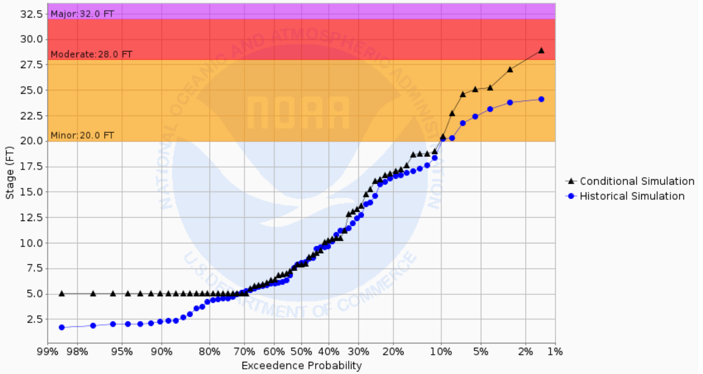
Chance of Exceeding River Stage at Wild Rice River at Hendrum (HNDM5) Forecast for the period 08/26/2024 - 11/24/2024 This is a conditional simulation based on the conditions as of 08/19/2024
