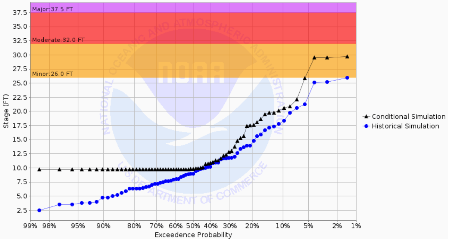
Chance of Exceeding River Stage at Red River of the North at Hillsboro 11ESE (Halstad MN) (HILN8) Forecast for the period 08/26/2024 - 11/24/2024 This is a conditional simulation based on the conditions as of 08/19/2024
