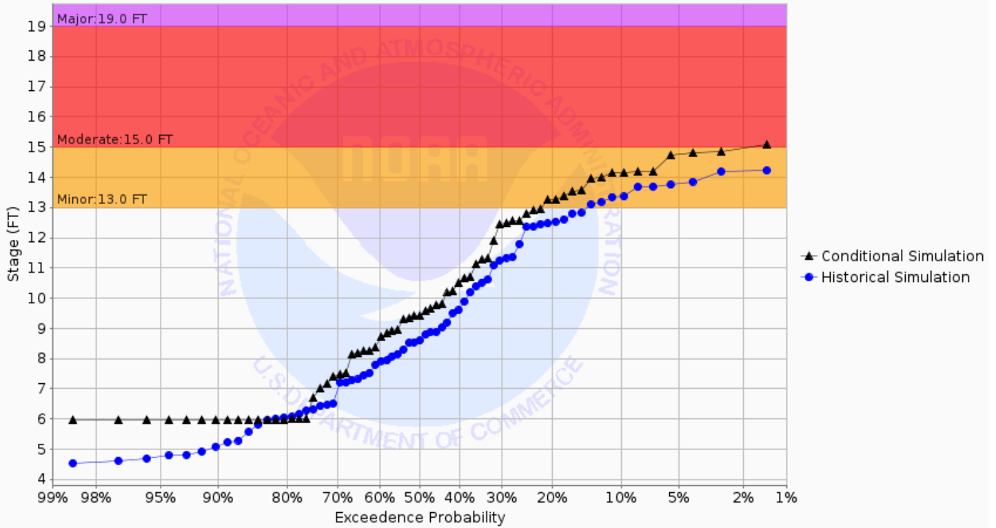
Chance of Exceeding River Stage at South Branch Buffalo River at Sabin 1E (SABM5) Forecast for the period 08/26/2024 - 11/24/2024 This is a conditional simulation based on the conditions as of 08/19/2024
