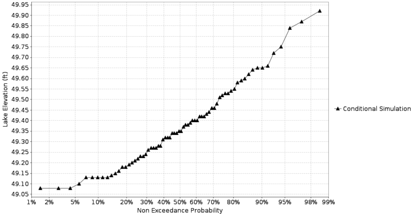
Probability of Falling to Low Lake Levels on the Devils Lake at Devils Lake SSW-Creel Bay (DCBN8) Forecast for the period 09/01/2024 - 11/30/2024 This is a conditional simulation based on the conditions as of 08/19/2024 Pumping schedule : 350cfs May 15 - Oct 30
