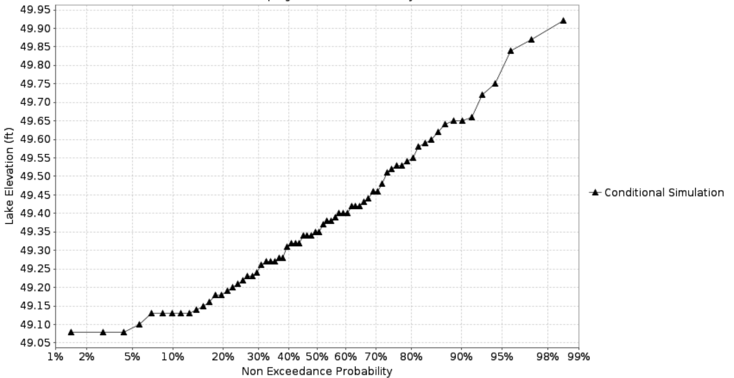
Probability of Falling to Low Lake Levels on the Eastern Stump Lake at Lakota 11S (ESLN8) Forecast for the period 09/01/2024 - 11/30/2024 This is a conditional simulation based on the conditions as of 08/19/2024 Pumping schedule : 350cfs May 15 - Oct 30
