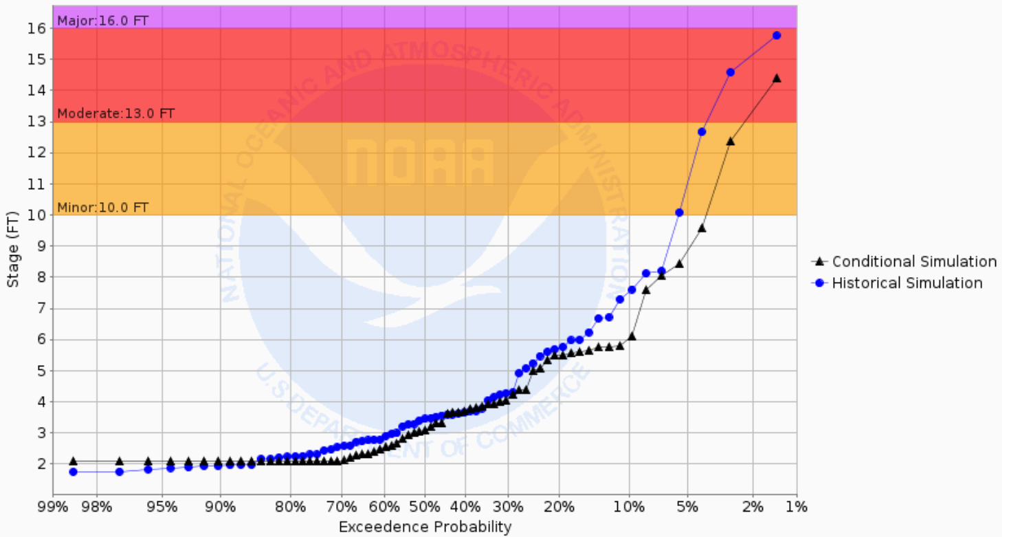
Chance of Exceeding River Stage at Goose River at Hillsboro (HGRN8) Forecast for the period 04/29/2024 - 07/28/2024 This is a conditional simulation based on the conditions as of 04/22/2024
