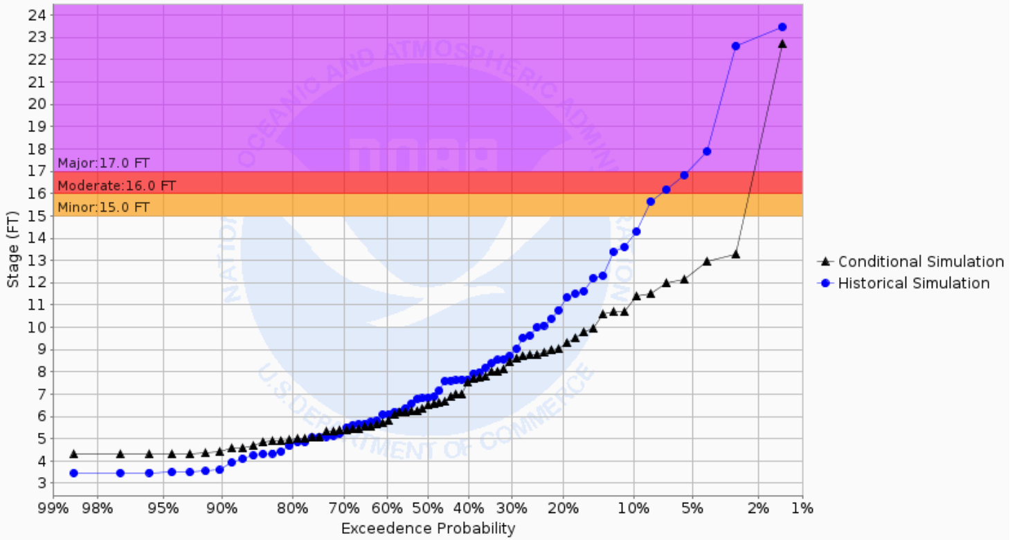
Chance of Exceeding River Stage at Sheyenne River at Valley City (VCRN8) Forecast for the period 04/29/2024 - 07/28/2024 This is a conditional simulation based on the conditions as of 04/22/2024
