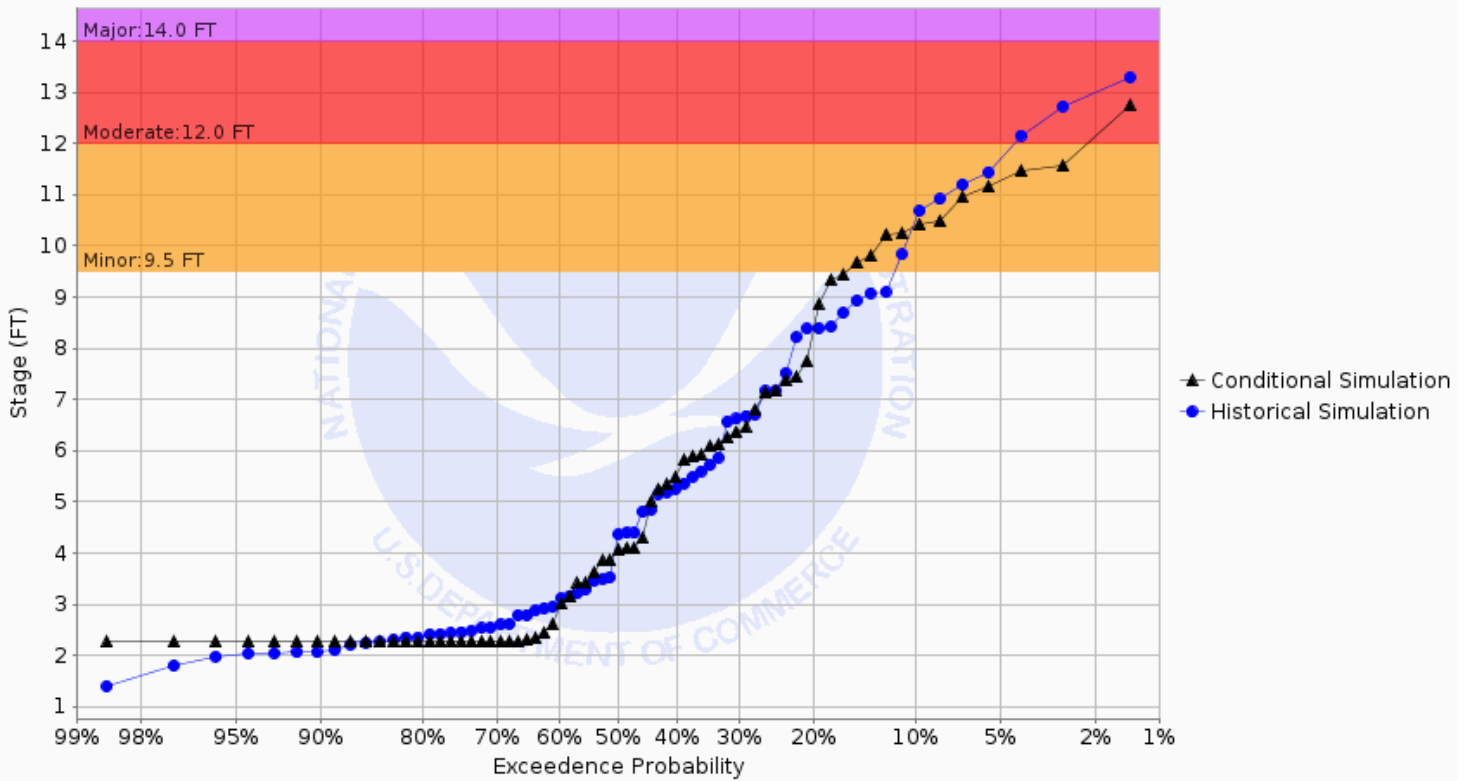
Chance of Exceeding River Stage at Maple River at Enderlin 1E (ENDN8) Forecast for the period 04/29/2024 - 07/28/2024 This is a conditional simulation based on the conditions as of 04/22/2024
