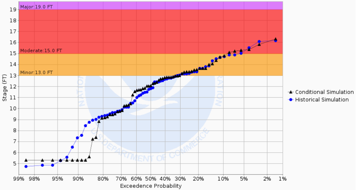
Chance of Exceeding River Stage at South Branch Buffalo River at Sabin 1E (SABM5) Forecast for the period 04/29/2024 - 07/28/2024 This is a conditional simulation based on the conditions as of 04/22/2024
