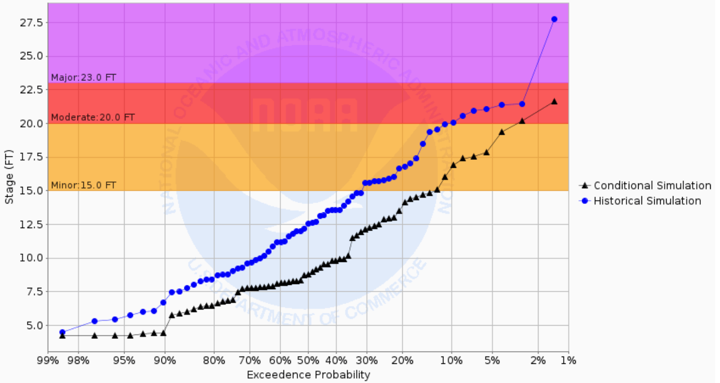
Chance of Exceeding River Stage at Red Lake River at Crookston (CRKM5) Forecast for the period 04/29/2024 - 07/28/2024 This is a conditional simulation based on the conditions as of 04/22/2024
