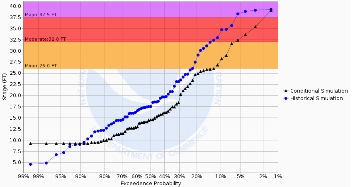
Chance of Exceeding River Stage at Red River of the North at Hillsboro 11ESE (Halstad MN) (HILN8) Forecast for the period 04/29/2024 - 07/28/2024 This is a conditional simulation based on the conditions as of 04/22/2024
