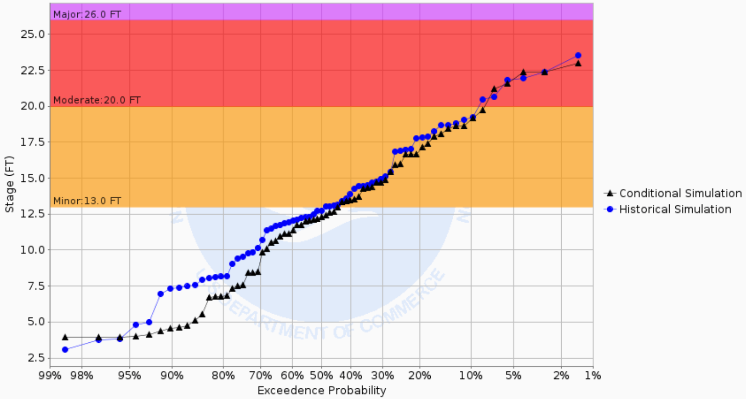
Chance of Exceeding River Stage at Buffalo River at Dilworth 7NE (DILM5) Forecast for the period 04/29/2024 - 07/28/2024 This is a conditional simulation based on the conditions as of 04/22/2024
