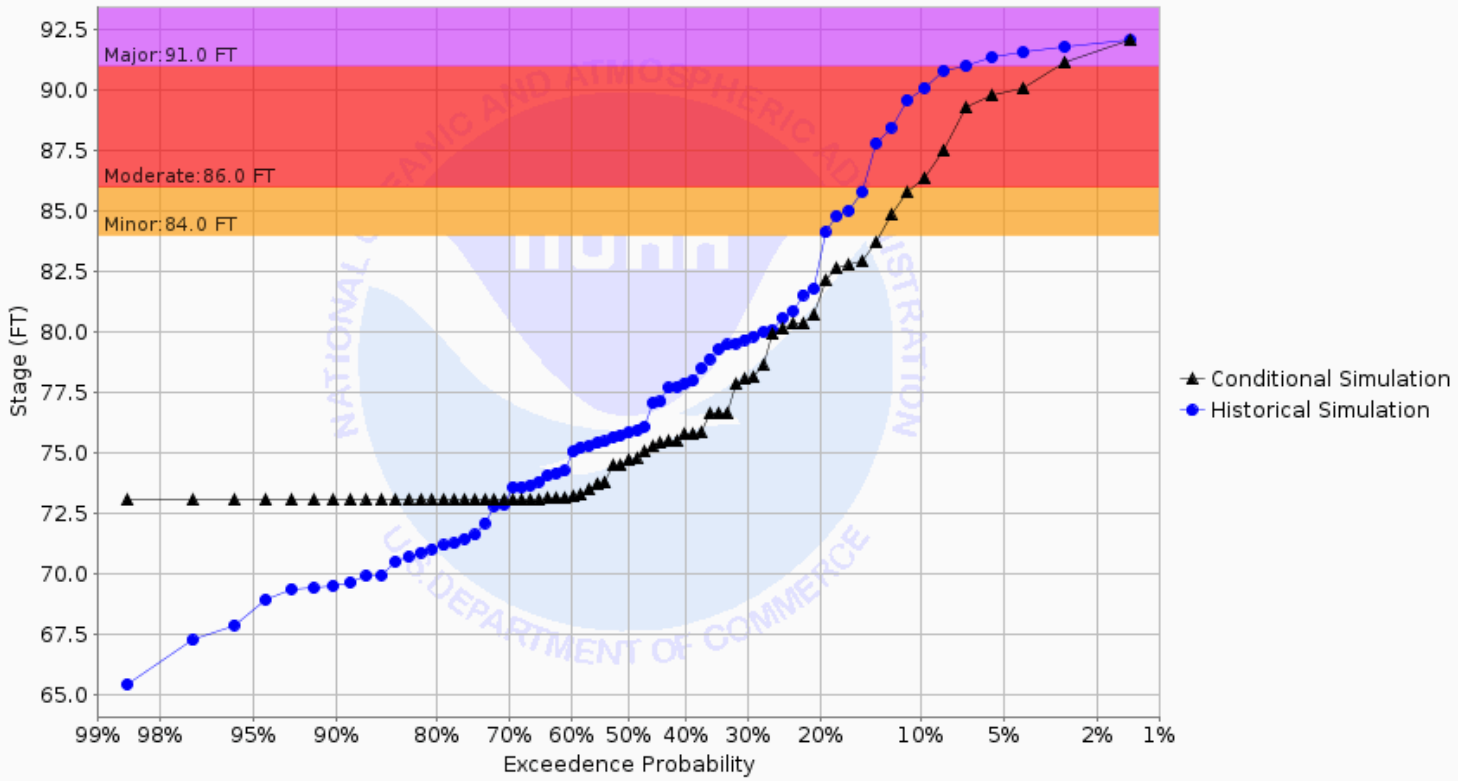
Chance of Exceeding River Stage at Sheyenne River at Harwood (HWDN8) Forecast for the period 04/29/2024 - 07/28/2024 This is a conditional simulation based on the conditions as of 04/22/2024
