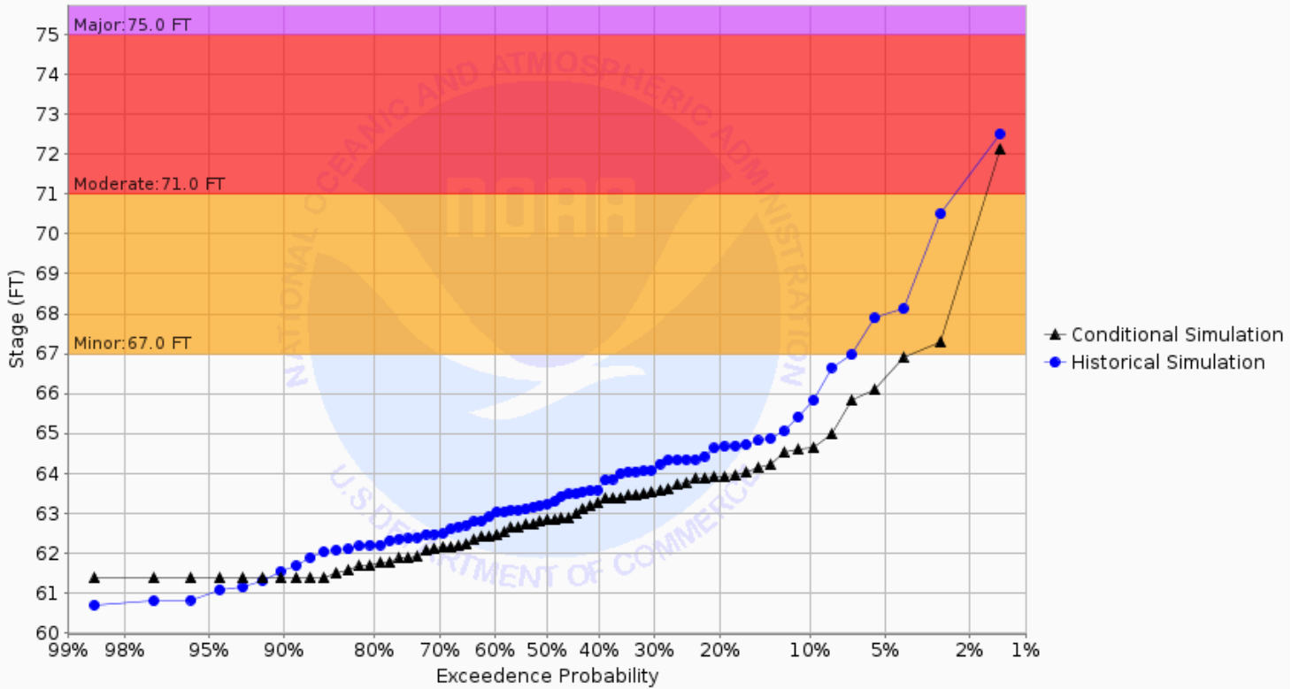
Chance of Exceeding River Stage at Snake River at Warren 3ENE-Morkassel Brdg (MKLM5) Forecast for the period 04/29/2024 - 07/28/2024 This is a conditional simulation based on the conditions as of 04/22/2024
