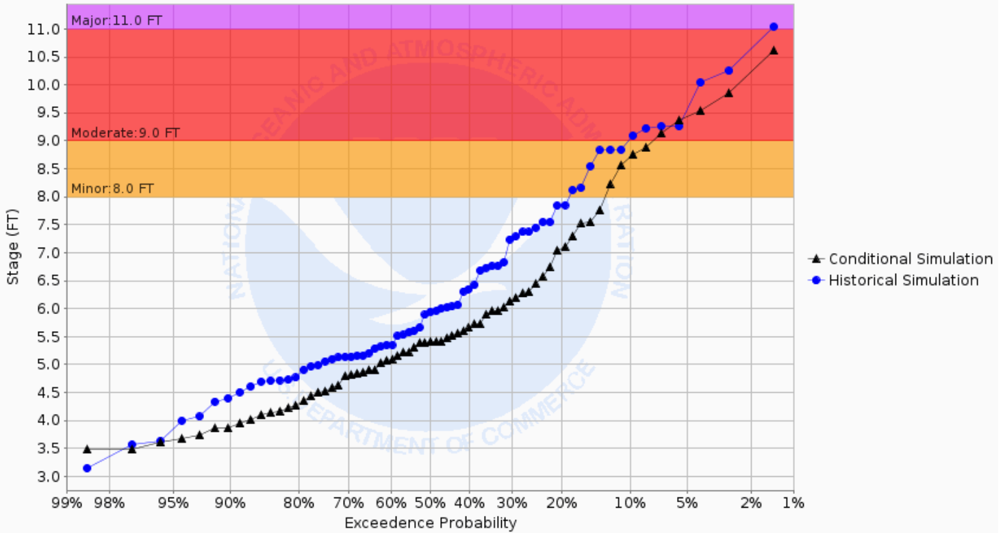
Chance of Exceeding River Stage at Buffalo River at Hawley 2SW (HWYM5) Forecast for the period 04/29/2024 - 07/28/2024 This is a conditional simulation based on the conditions as of 04/22/2024
