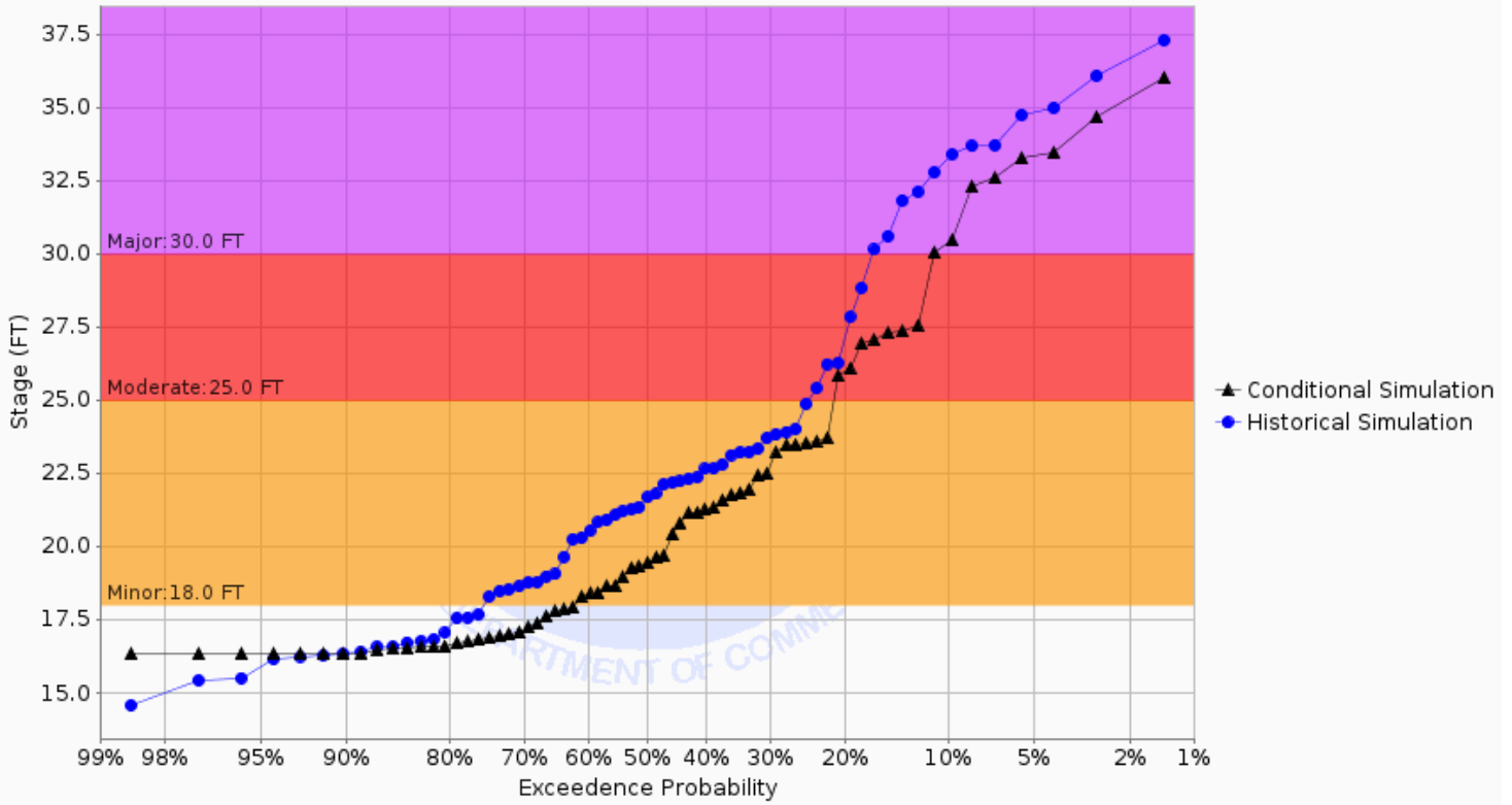
Chance of Exceeding River Stage at Red River of the North at Fargo WTP (FGON8) Forecast for the period 04/29/2024 - 07/28/2024 This is a conditional simulation based on the conditions as of 04/22/2024
