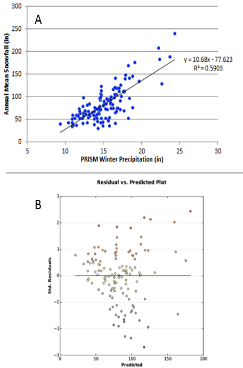
Figure 6. (a) Scatterplot showing the distribution of Annual Mean Snowfall vs. PRISM gridded winter precipitation values, and (b) the scatterplot of the standard deviation of the residuals from the OLR model output vs the predicted value.
