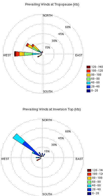
Figure 4: Wind Roses depicting most frequent wind direction (angle) and speed (color) at the tropopause (top) and top of the inversion (bottom).
