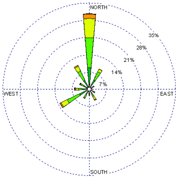
Santa Fe (23049) 1985-2005 January - All hours Average Speed - 8.37 kt Calms: 7.11%
