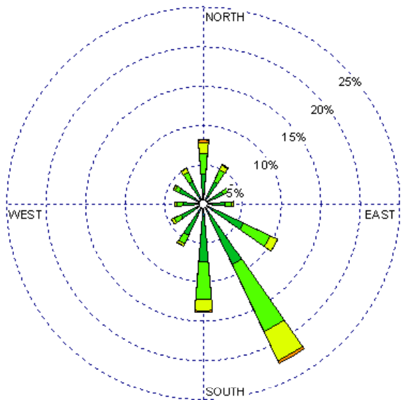
Roswell (23009) 1985-2005 September - All hours Average Speed= 7.13 kt
