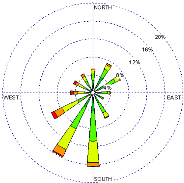
Las Vegas (23054) 1985-2005 February - All hours Average Speed - 9.23 kt
