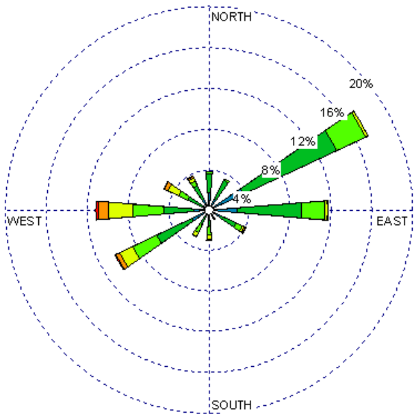
Farmington (23090) 1985-2005 October - All hours Average Speed - 5.58 kt
