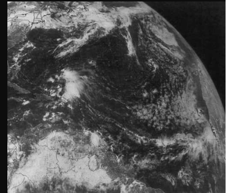
July 20, 1981 1600 UTC
