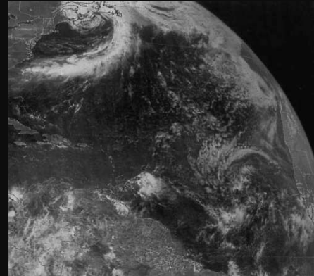
July 15, 1981 1600 UTC
