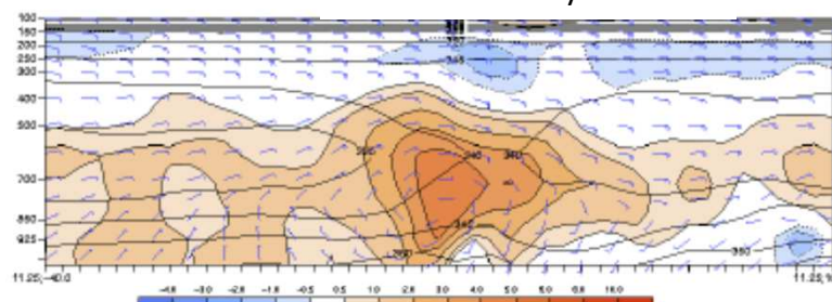
Relative Humidity
