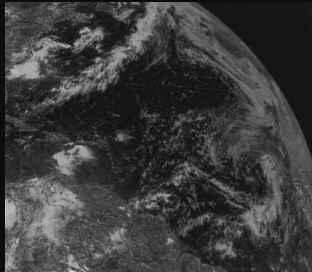
July 17, 1981 1600 UTC
